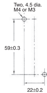
Mounting Holes
