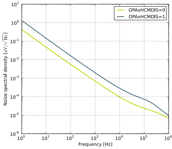
Figure 3.27. OPAMP Voltage Noise Spectral Density (Non-Unity Gain)
