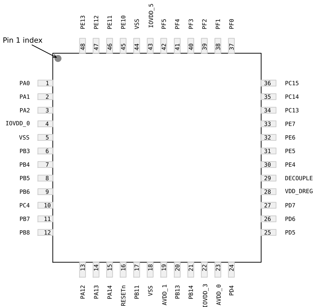
Figure 4.1. EFM32TG822 Pinout (top view, not to scale)
