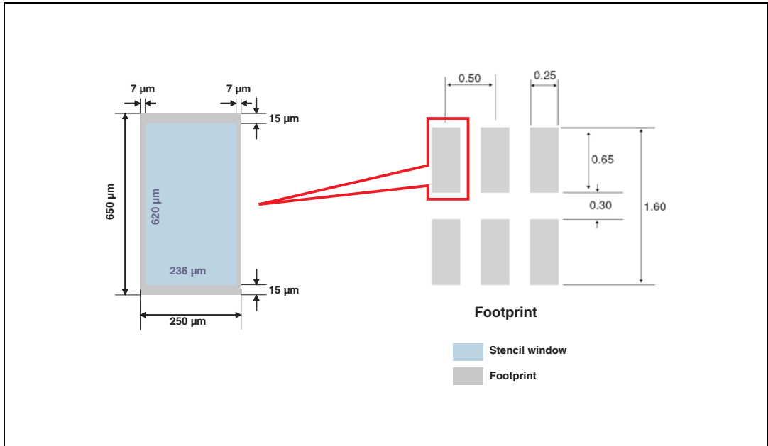
Figure 18. Recommended stencil window position for μQFN-6L
