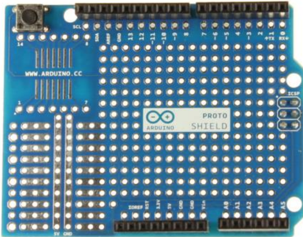
Proto Shield R3 mounted Front
