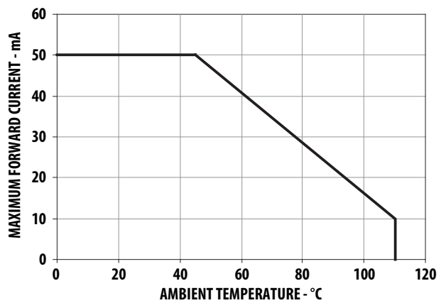
Figure 4a. Maximum Forward Current Vs. Ambient Temperature. Derated Based on T_{JMAX} = 125^{\circ}C , R\theta_{JA} = 300^{\circ}C/W
