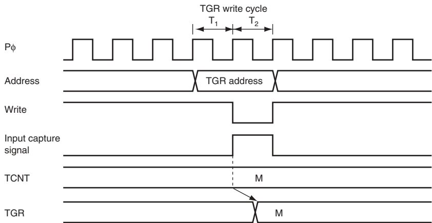
Figure 10.51 Conflict between TGR Write and Input Capture
