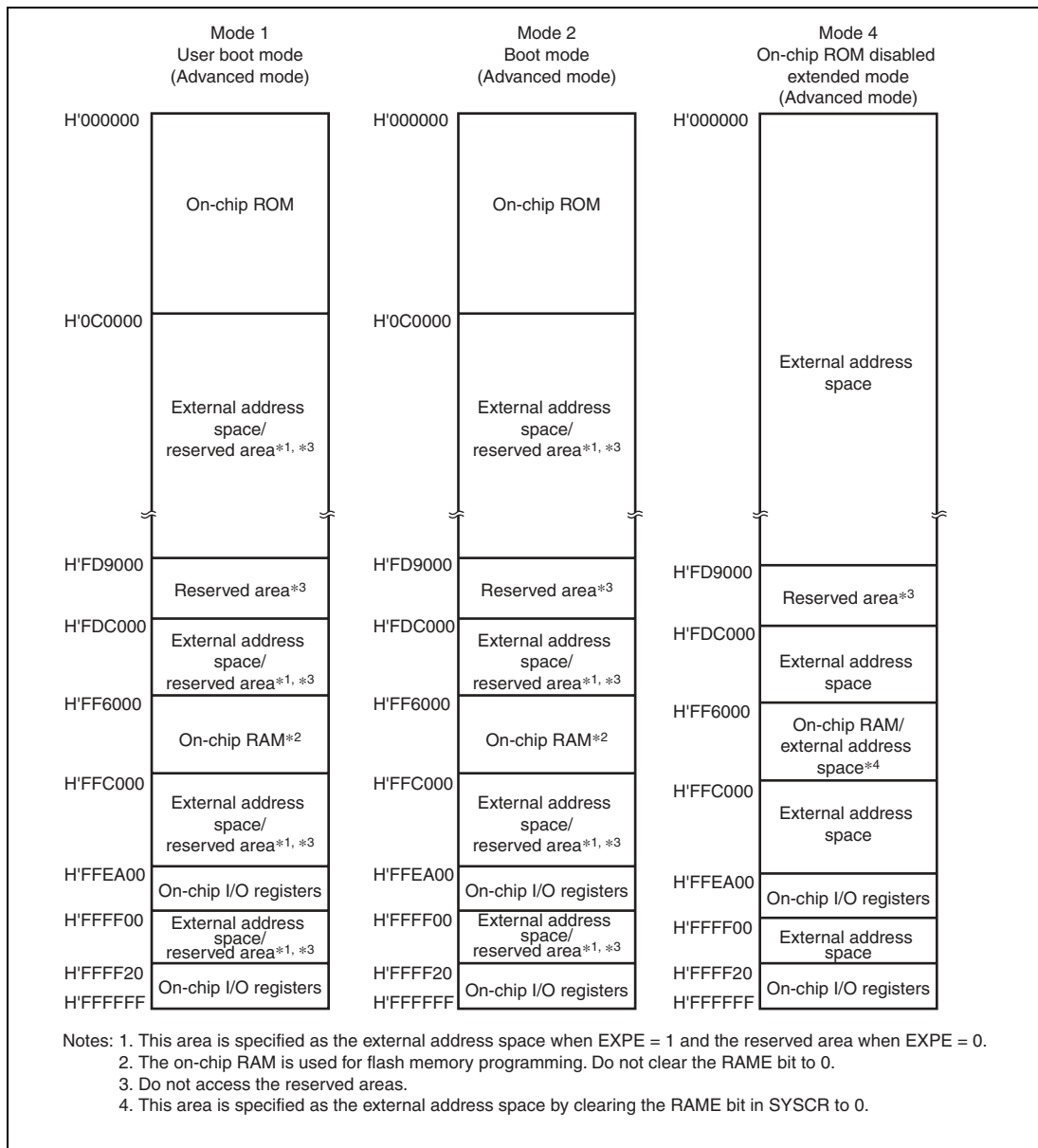
Figure 3.1 Address Map (1)
