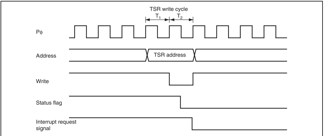
Figure 10.42 Timing for Status Flag Clearing by CPU
