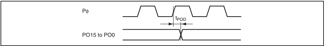
Figure 22.28 PPG Output Timing
