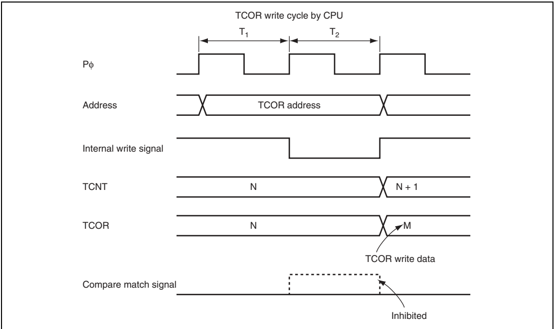
Figure 12.15 Conflict between TCOR Write and Compare Match
