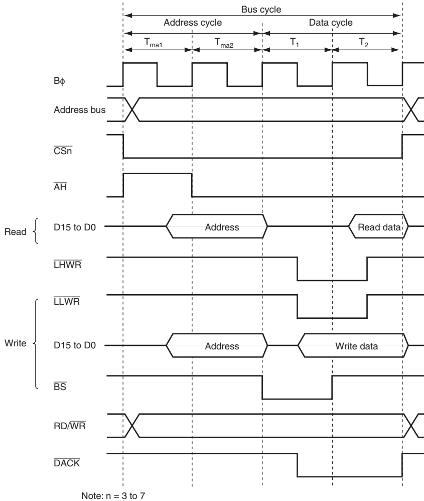
Figure 6.31 16-Bit Access Space Access Timing (ABWHn = 0, ABWLn = 1)
