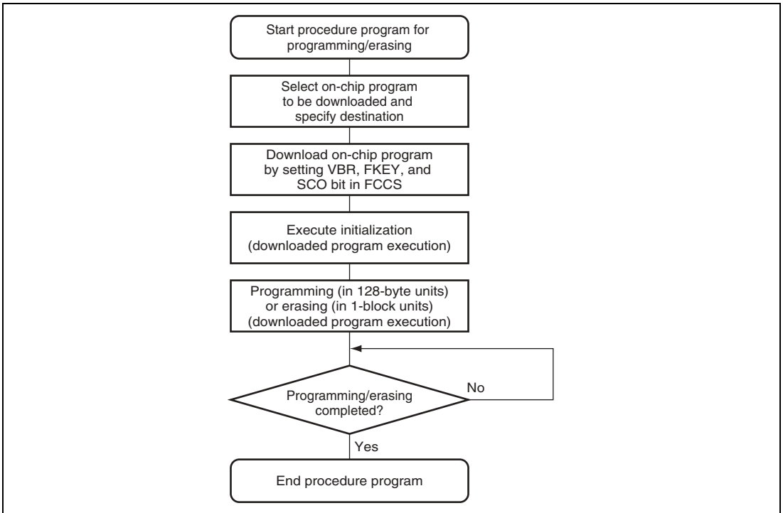
Figure 18.5 Procedure for Creating Procedure Program
