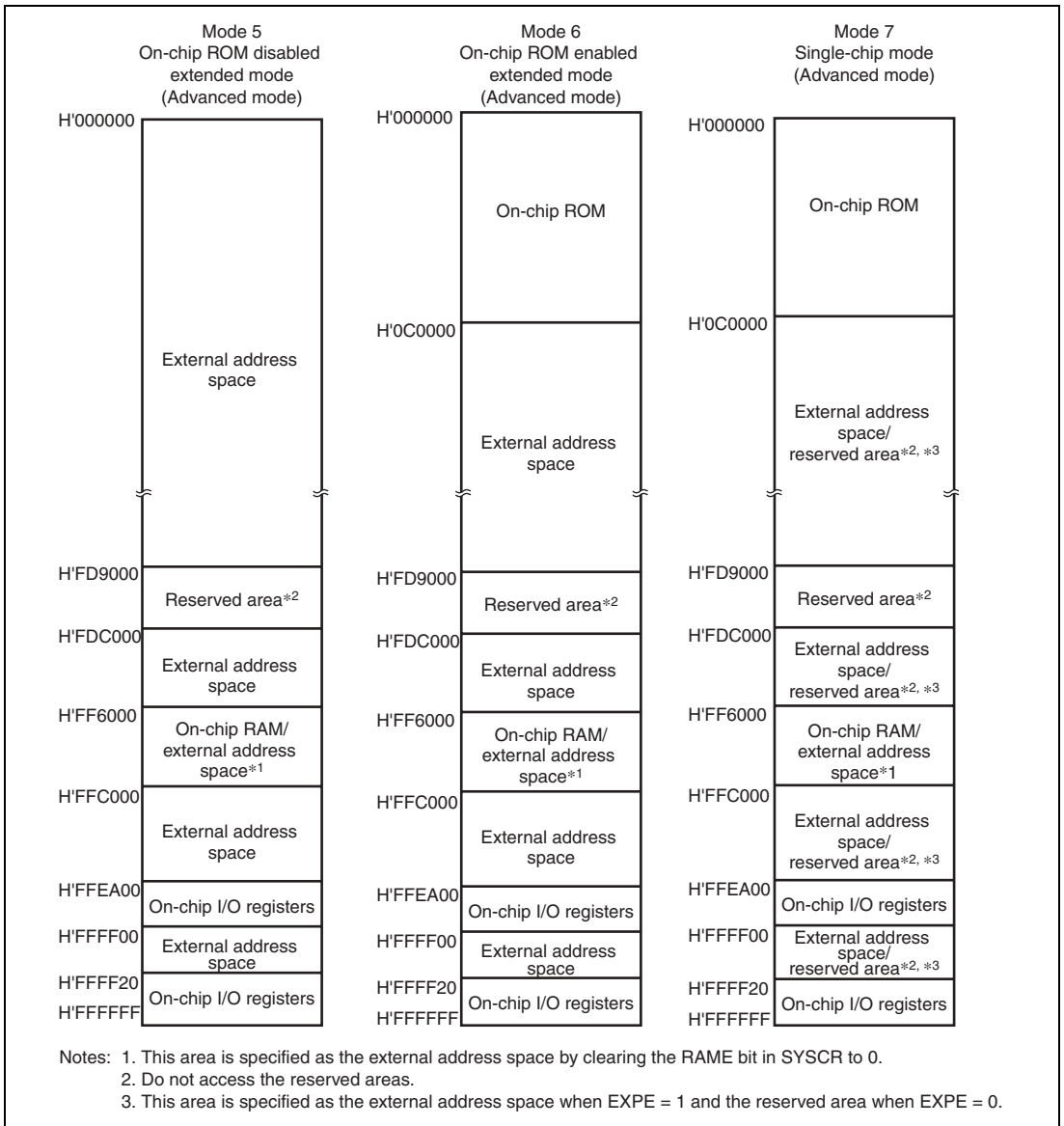
Figure 3.2 Address Map (2)
