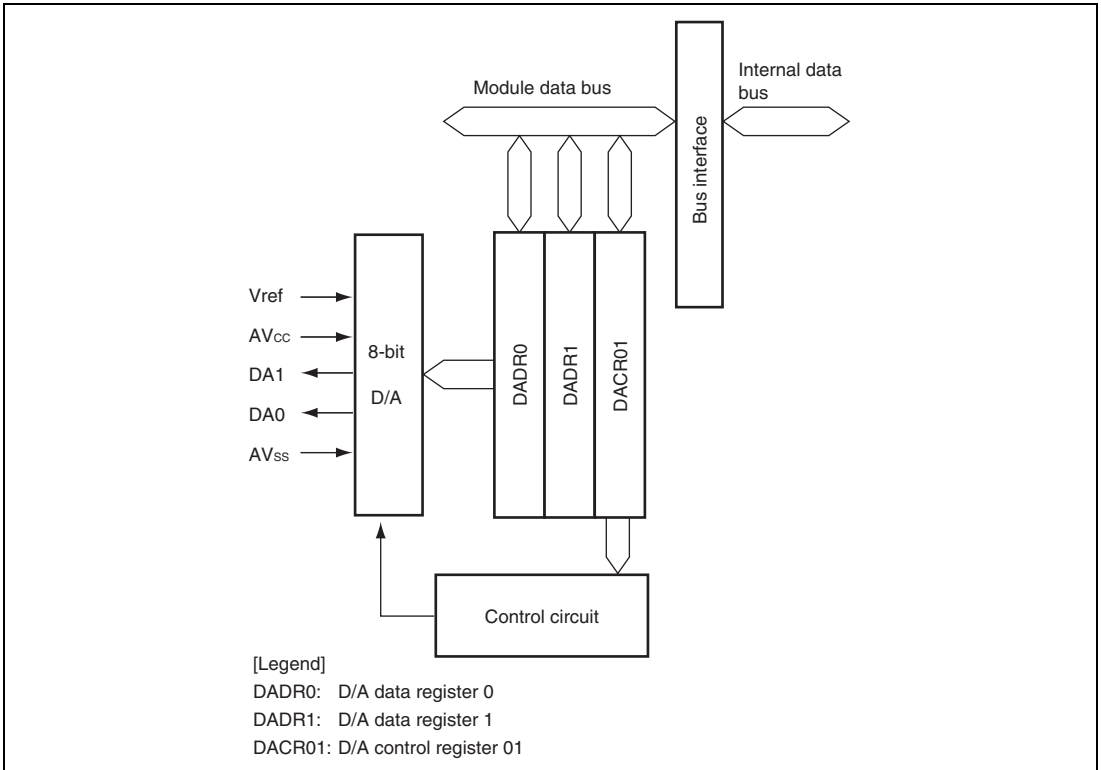
Figure 16.1 Block Diagram of D/A Converter
