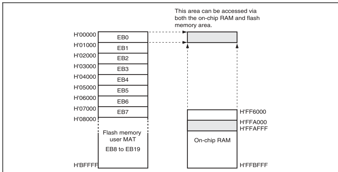
Figure 18.20 Address Map of Overlaid RAM Area
