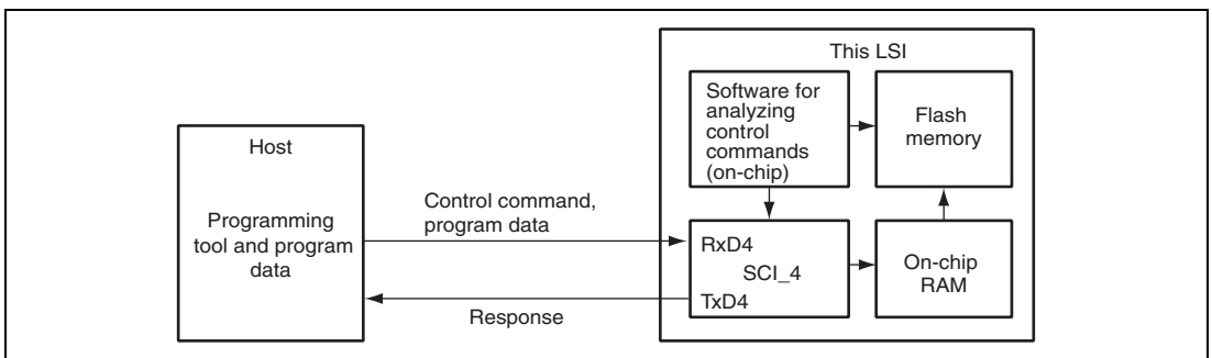
Figure 18.6 System Configuration in Boot Mode
