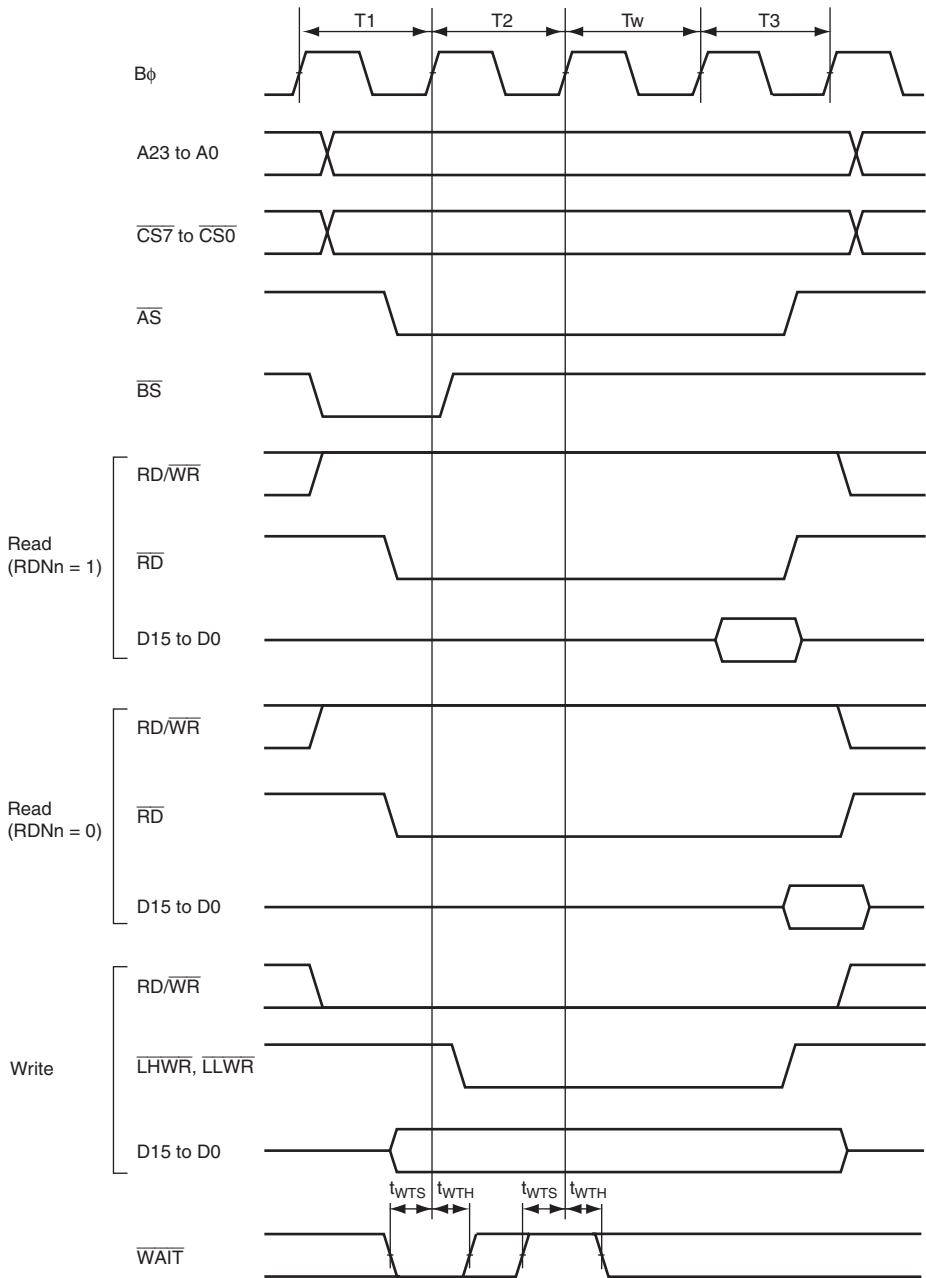
Figure 22.10 Basic Bus Timing: Three-State Access, One Wait
