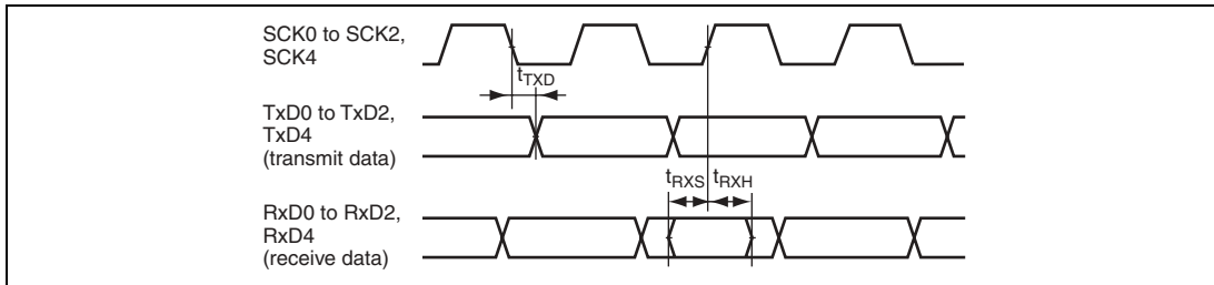
Figure 22.34 SCI Input/Output Timing: Clocked Synchronous Mode
