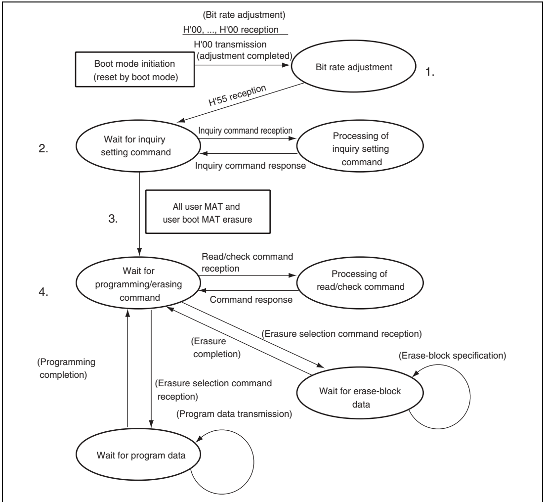
Figure 18.8 Boot Mode State Transition Diagram
