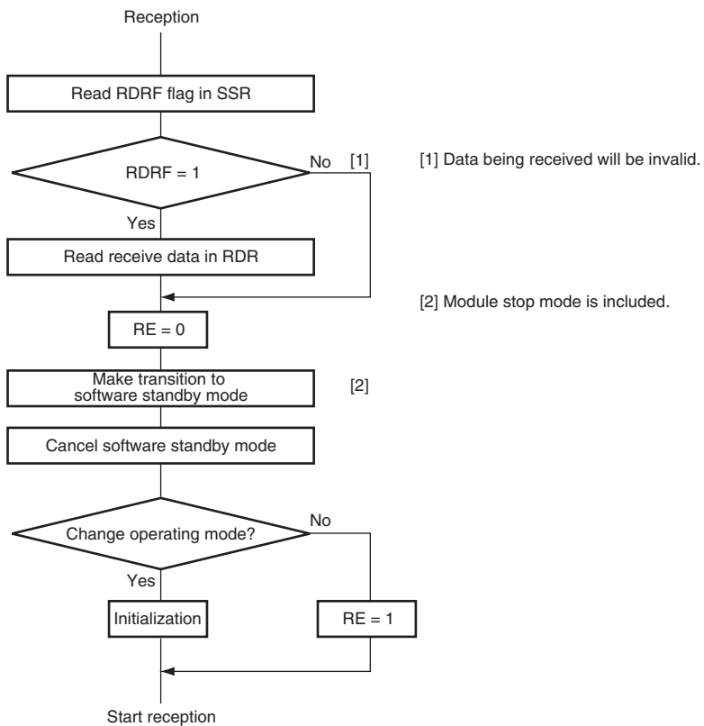
Figure 14.37 Sample Flowchart for Mode Transition during Reception
