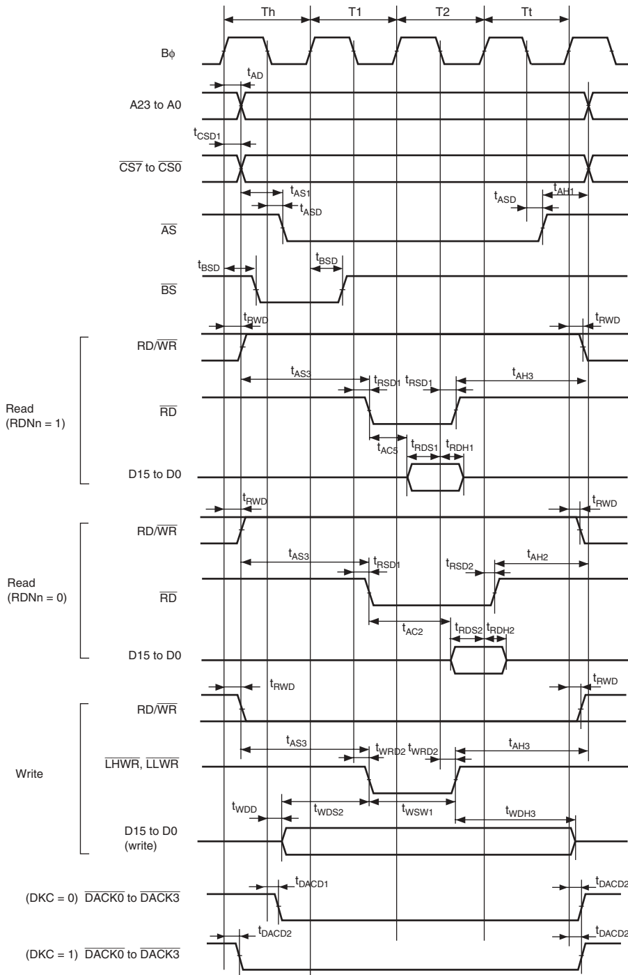
Figure 22.11 Basic Bus Timing: 2-State Access ( \overline{CS} Assertion Period Extended)
