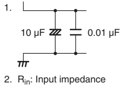
Figure 15.9 Example of Analog Input Protection Circuit
