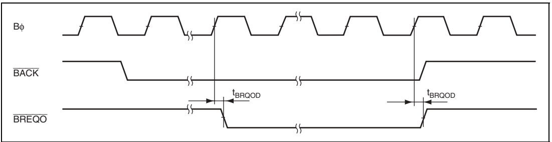
Figure 22.20 External Bus Request Output Timing
