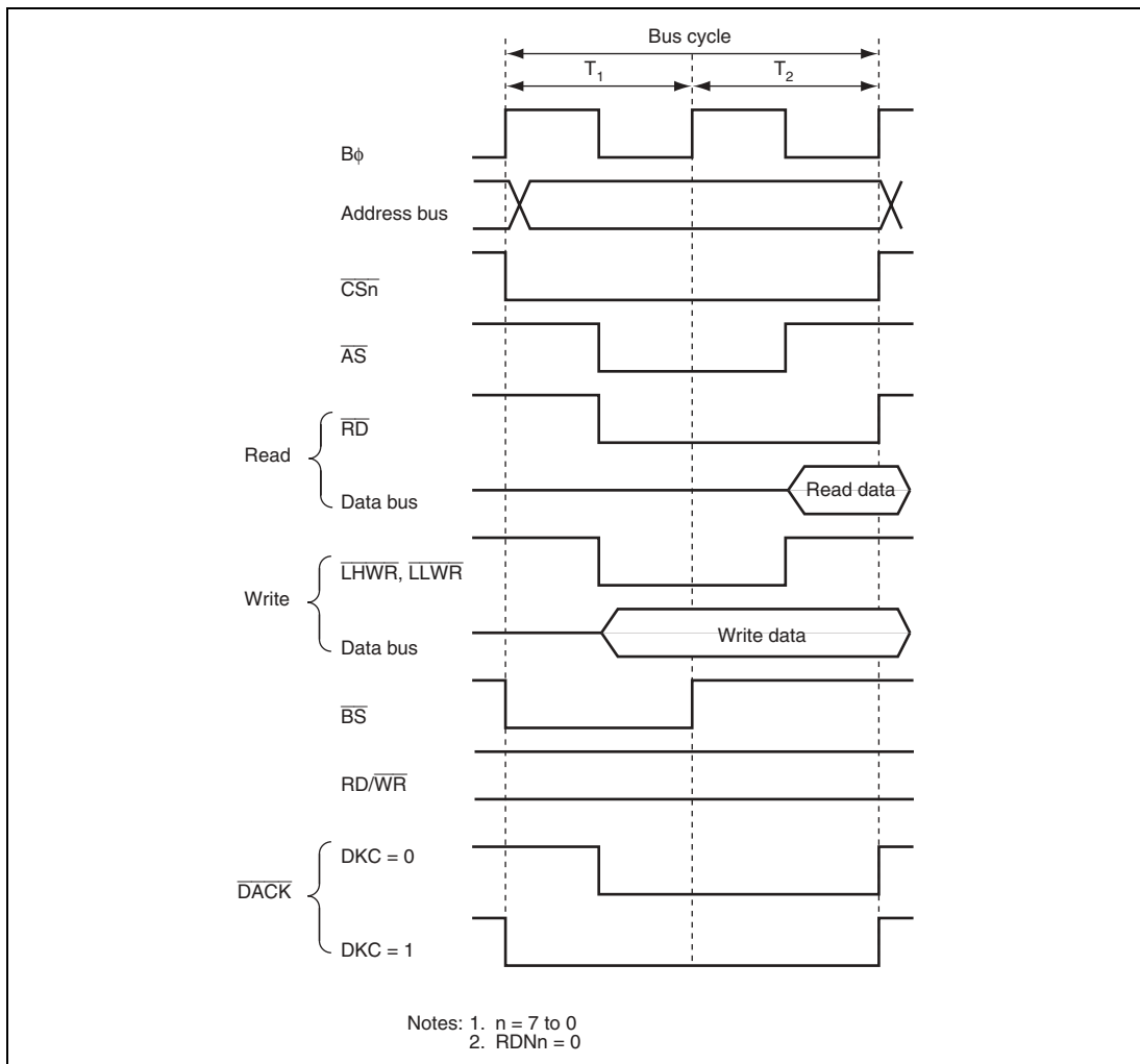
Figure 6.23 \overline{\text{DACK}} Signal Output Timing
