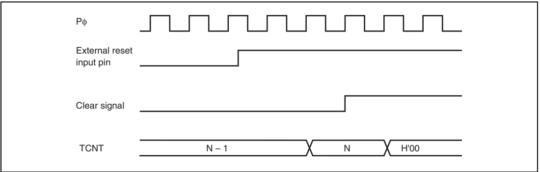
Figure 12.11 Timing of Clearance by External Reset (High Level)
