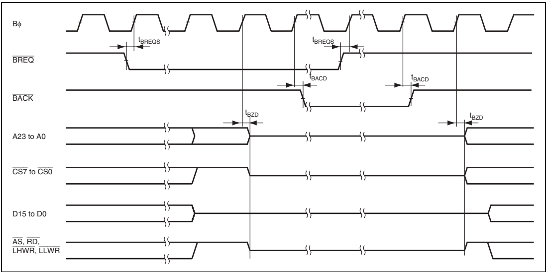
Figure 22.19 External Bus Release Timing
