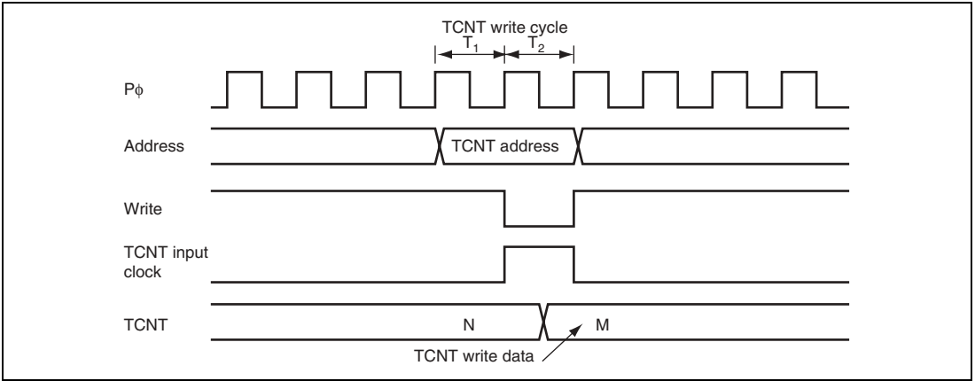
Figure 10.47 Conflict between TCNT Write and Increment Operations
