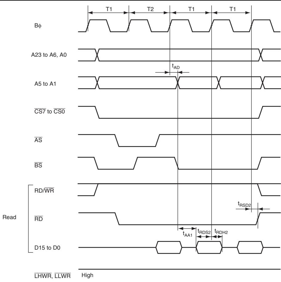
Figure 22.15 Burst ROM Access Timing: 1-State Burst Access
