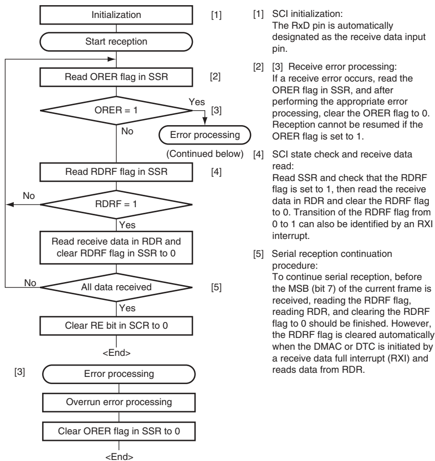
Figure 14.19 Sample Serial Reception Flowchart
