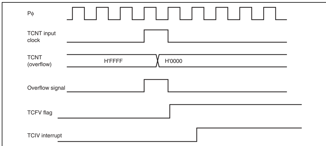
Figure 10.40 TCIV Interrupt Setting Timing
