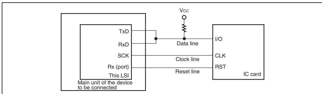
Figure 14.21 Pin Connection for Smart Card Interface
