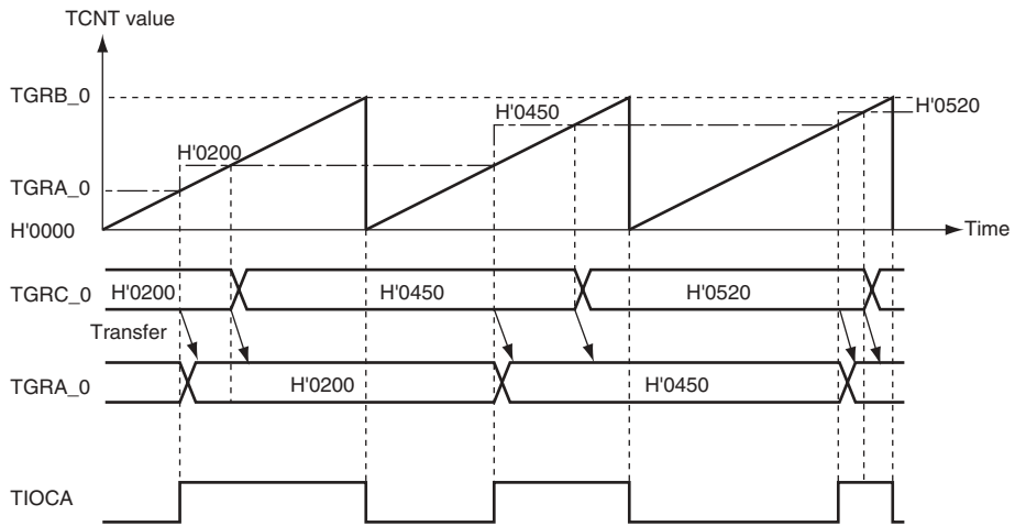
Figure 10.15 Example of Buffer Operation (1)
