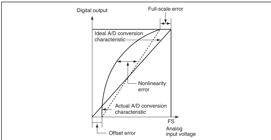
Figure 15.7 A/D Conversion Accuracy Definitions
