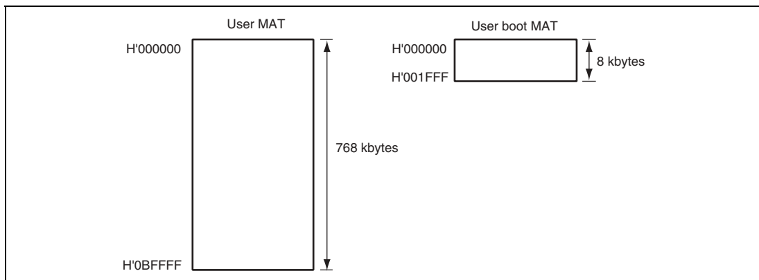
Figure 18.3 Memory MAT Configuration
