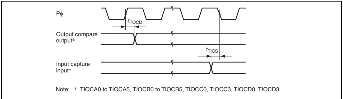
Figure 22.26 TPU Input/Output Timing
