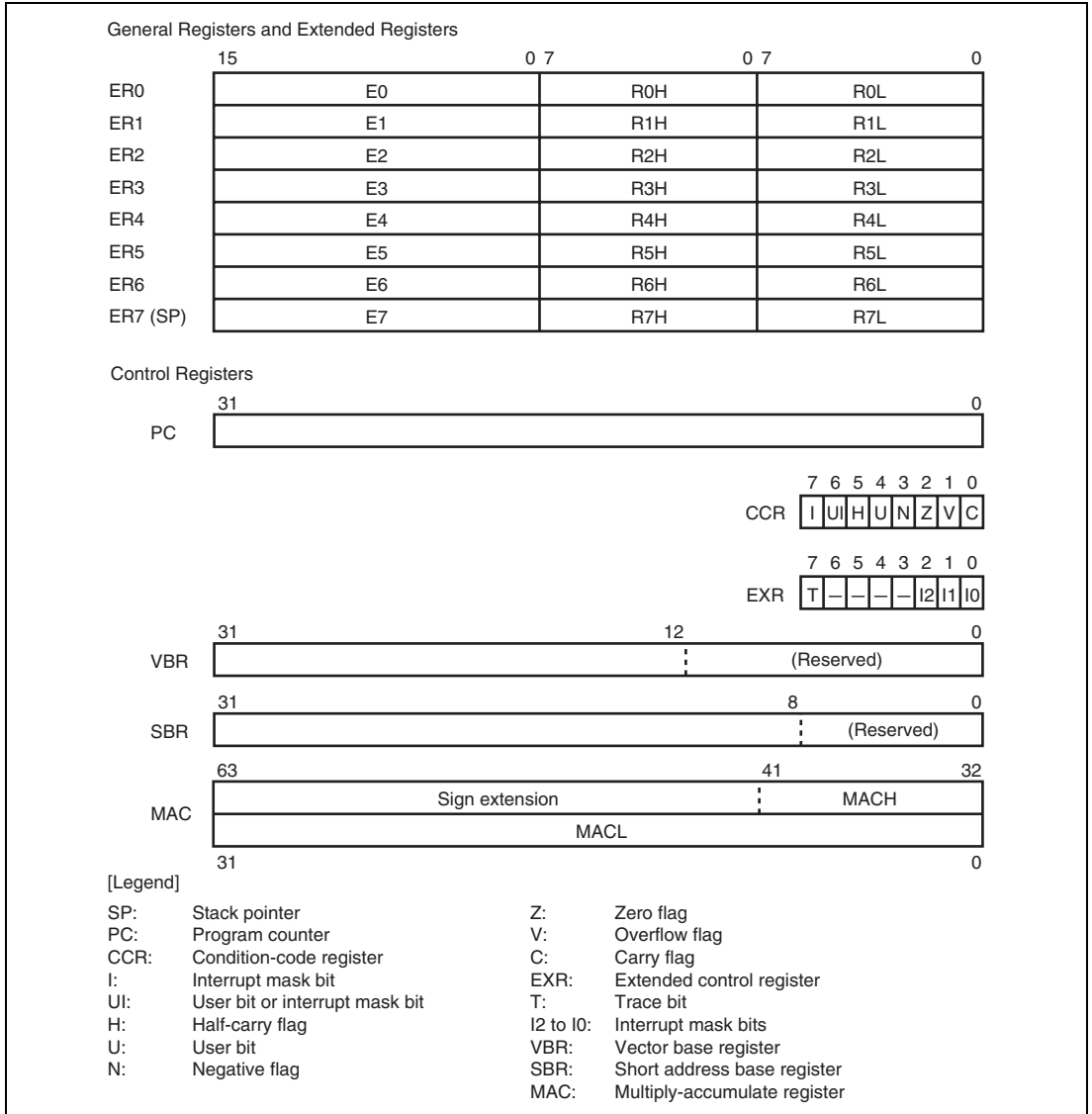
Figure 2.9 CPU Registers
