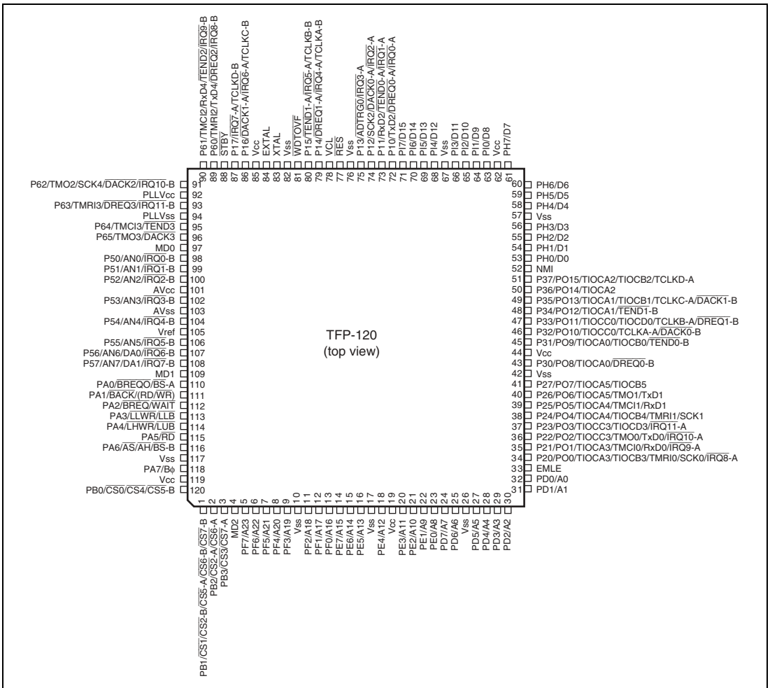
Figure 1.2 Pin Assignments
