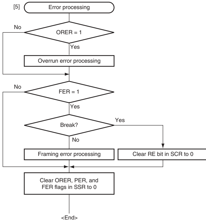
Figure 14.13 Sample Multiprocessor Serial Reception Flowchart (2)
