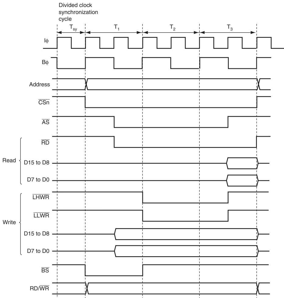
Figure 6.6 System Clock: External Bus Clock = 2:1, External 3-State Access
