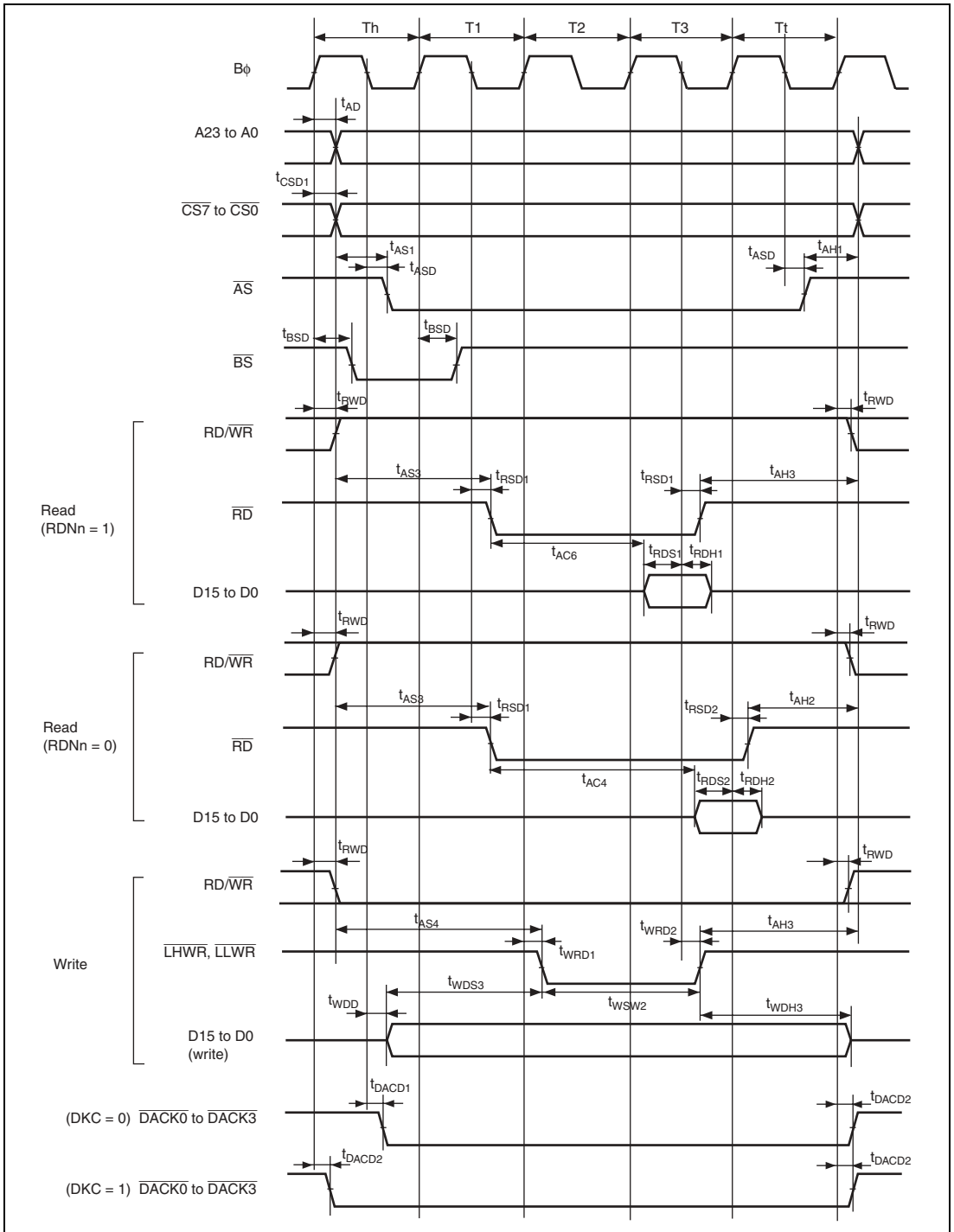
Figure 22.12 Basic Bus Timing: 3-State Access ( \overline{CS} Assertion Period Extended)
