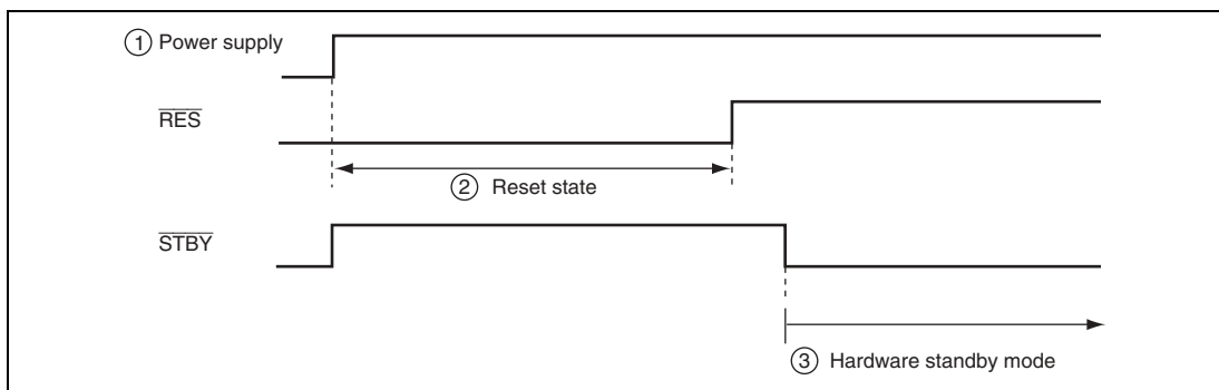
Figure 20.4 Timing Sequence at Power-On
