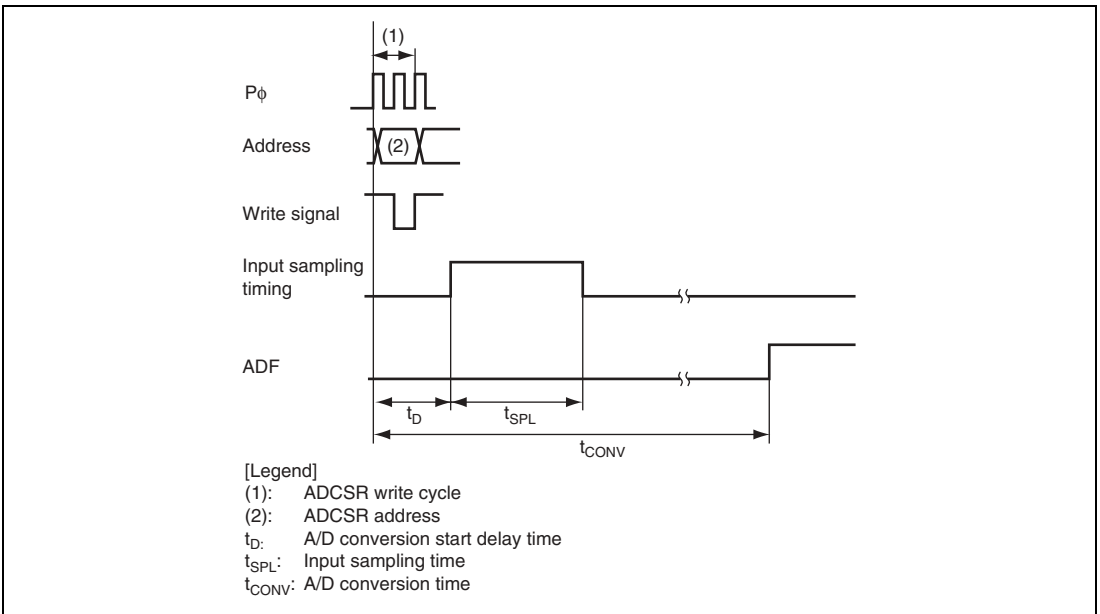
Figure 15.4 A/D Conversion Timing
