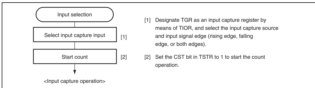
Figure 10.8 Example of Setting Procedure for Input Capture Operation
