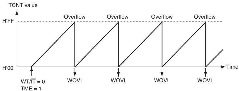
Figure 13.3 Operation in Interval Timer Mode
