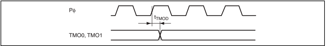
Figure 22.29 8-Bit Timer Output Timing
