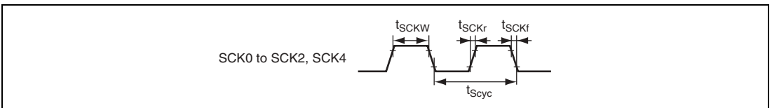
Figure 22.33 SCK Clock Input Timing
