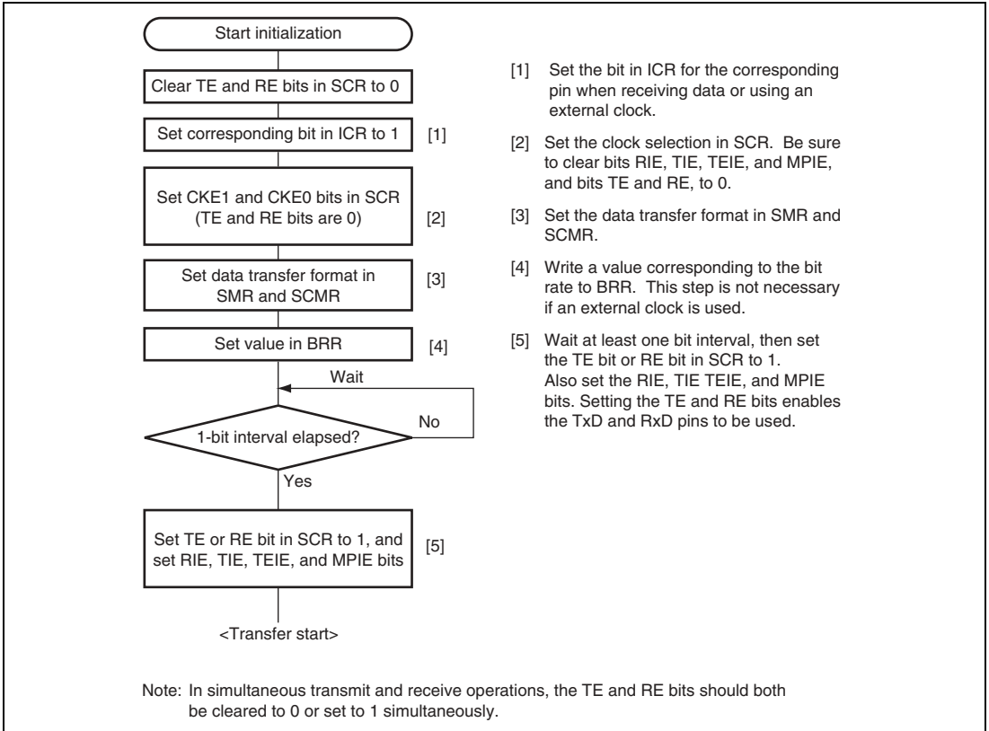
Figure 14.15 Sample SCI Initialization Flowchart
