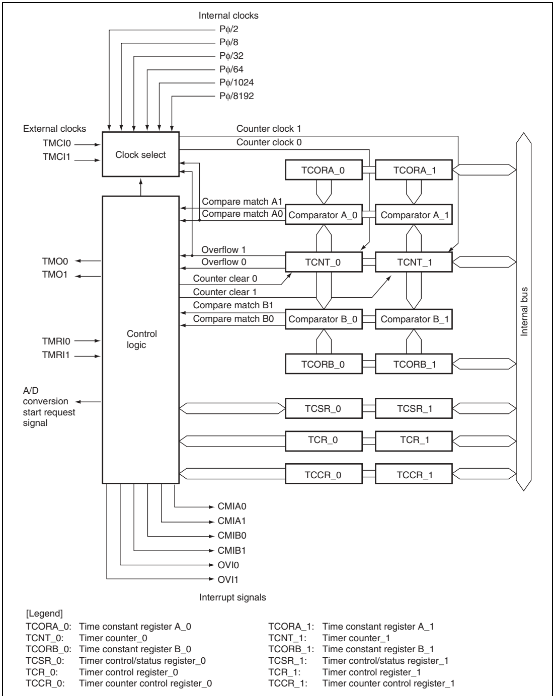
Figure 12.1 Block Diagram of 8-Bit Timer Module (Unit 0)
