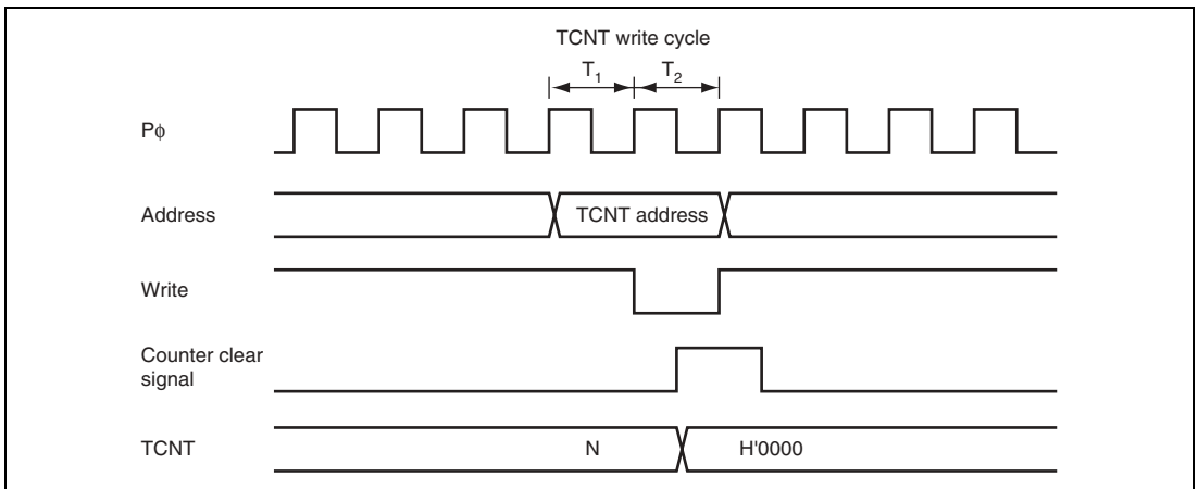
Figure 10.46 Conflict between TCNT Write and Clear Operations
