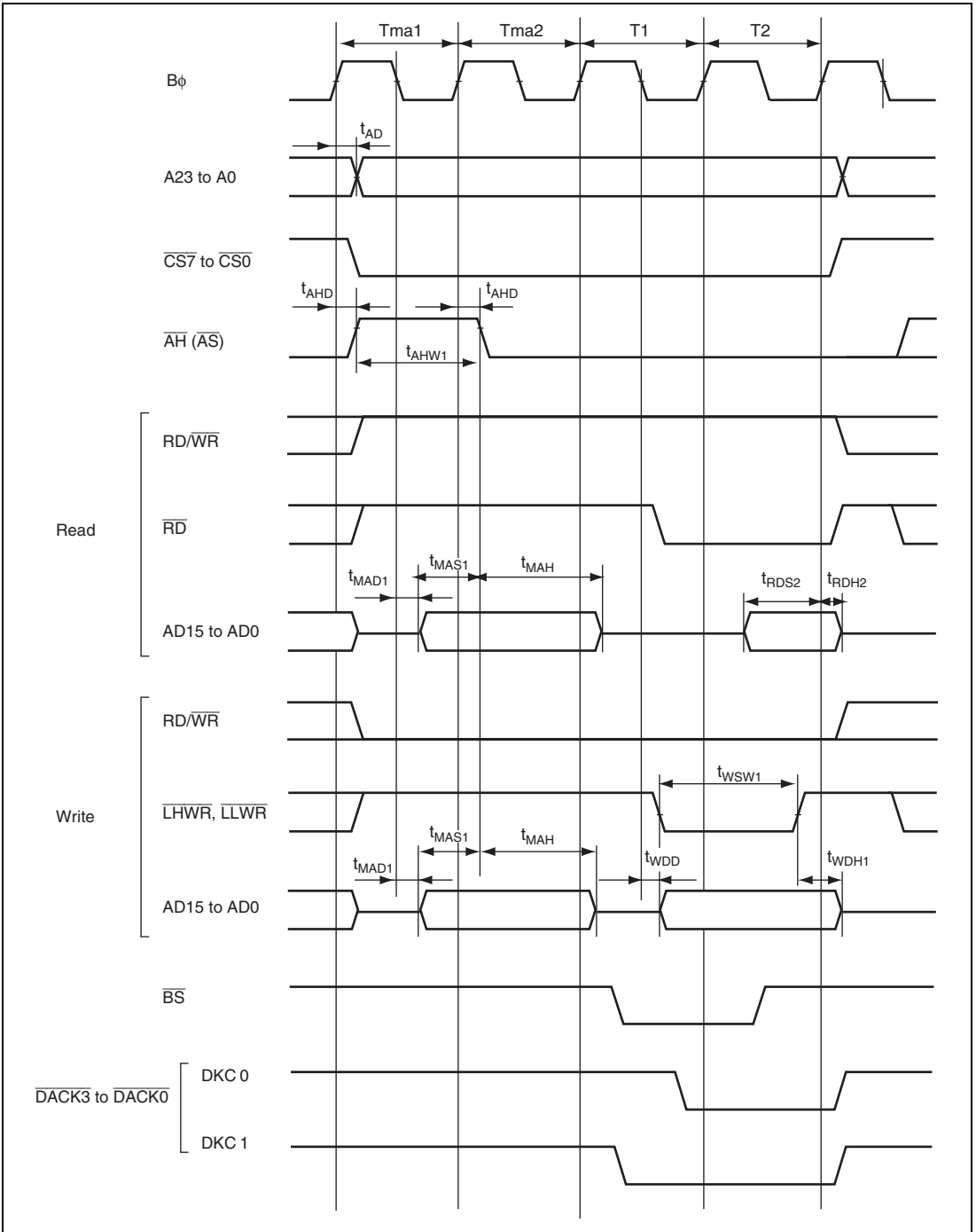
Figure 22.17 Address/Data Multiplexed Access Timing (No Wait) (Basic, 4-State Access)
