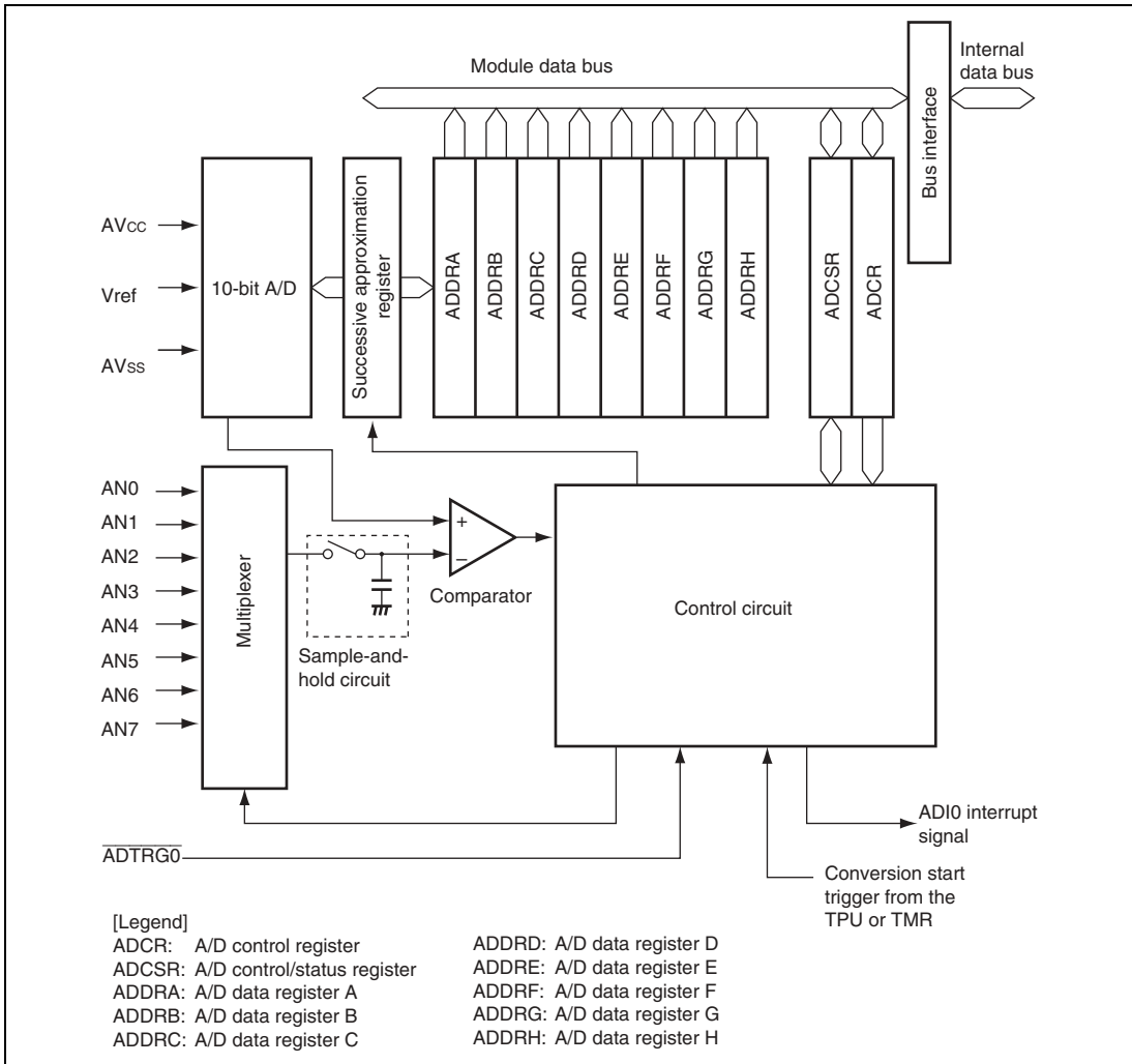
Figure 15.1 Block Diagram of A/D Converter
