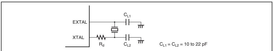
Figure 19.2 Connection of Crystal Resonator (Example)
