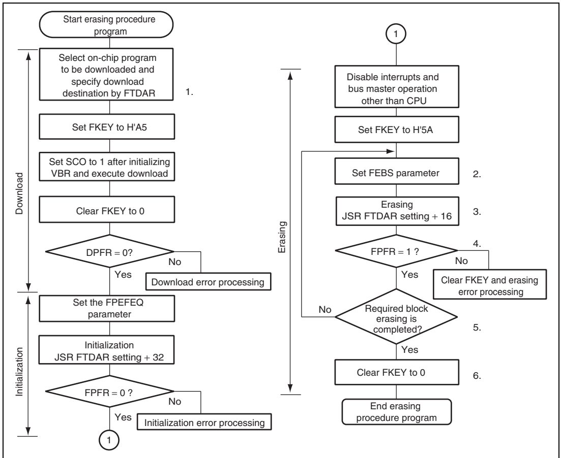
Figure 18.14 Erasing Procedure in User Program Mode
