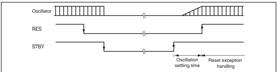
Figure 20.3 Hardware Standby Mode Timing
