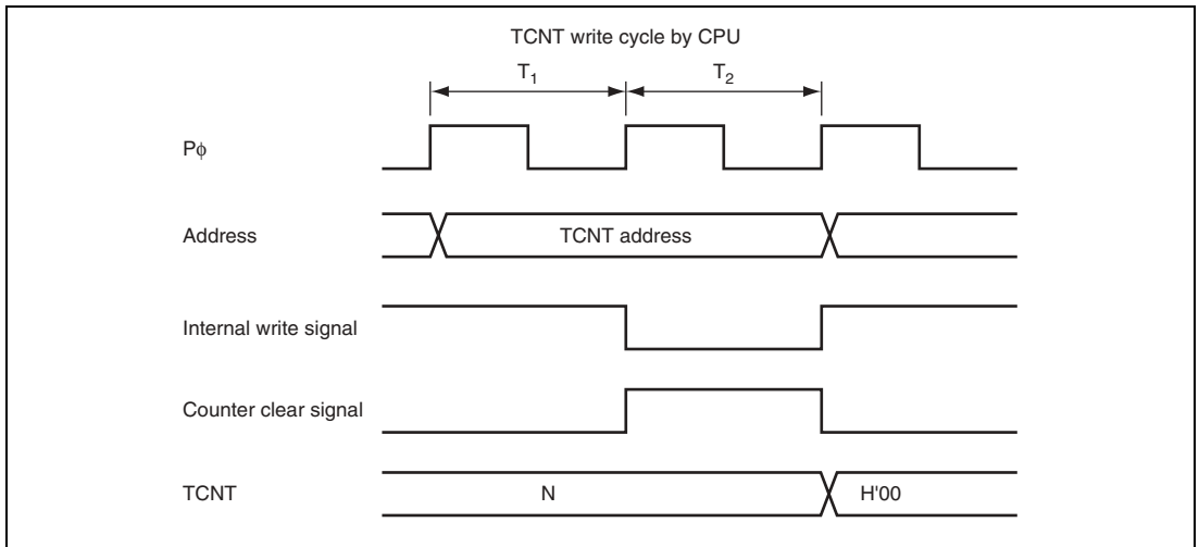
Figure 12.13 Conflict between TCNT Write and Clear
