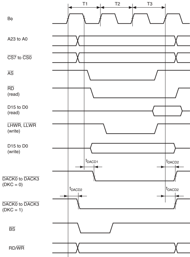
Figure 22.24 DMAC Single-Address Transfer Timing: 3-State Access
