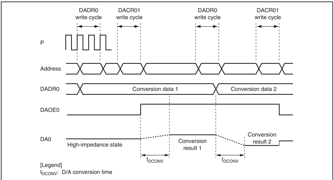
Figure 16.2 Example of D/A Converter Operation
