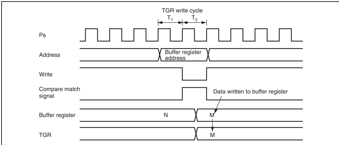
Figure 10.49 Conflict between Buffer Register Write and Compare Match
