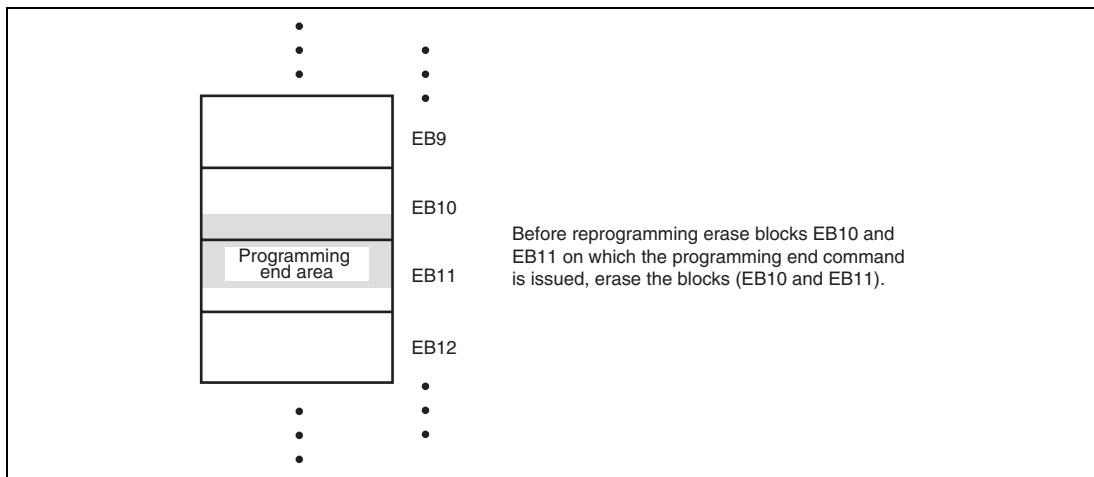
Figure 18.9 Example of Erase Block Including Programmed Area
