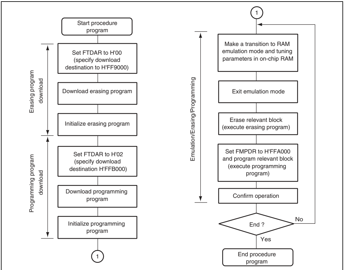
Figure 18.15 Repeating Procedure of Erasing, Programming, and RAM Emulation in User Program Mode
