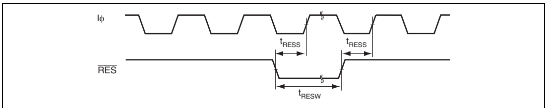
Figure 22.6 Reset Input Timing
