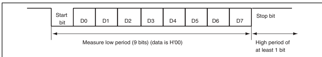
Figure 18.7 Automatic-Bit-Rate Adjustment Operation
