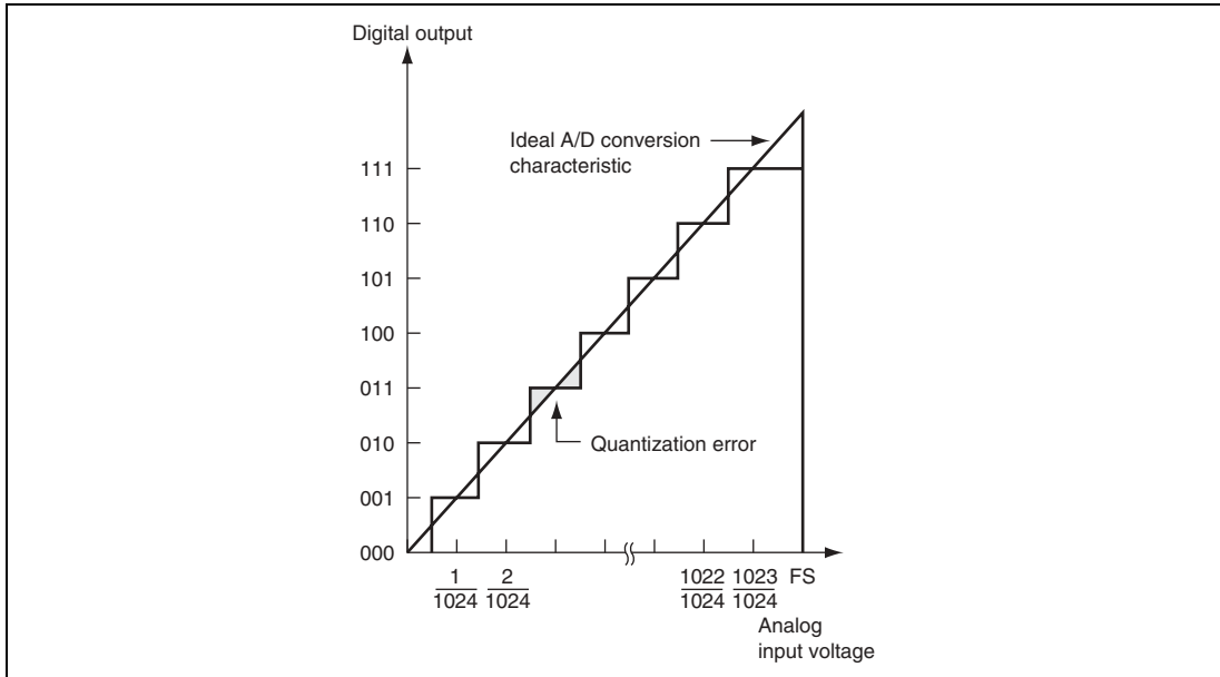
Figure 15.6 A/D Conversion Accuracy Definitions
