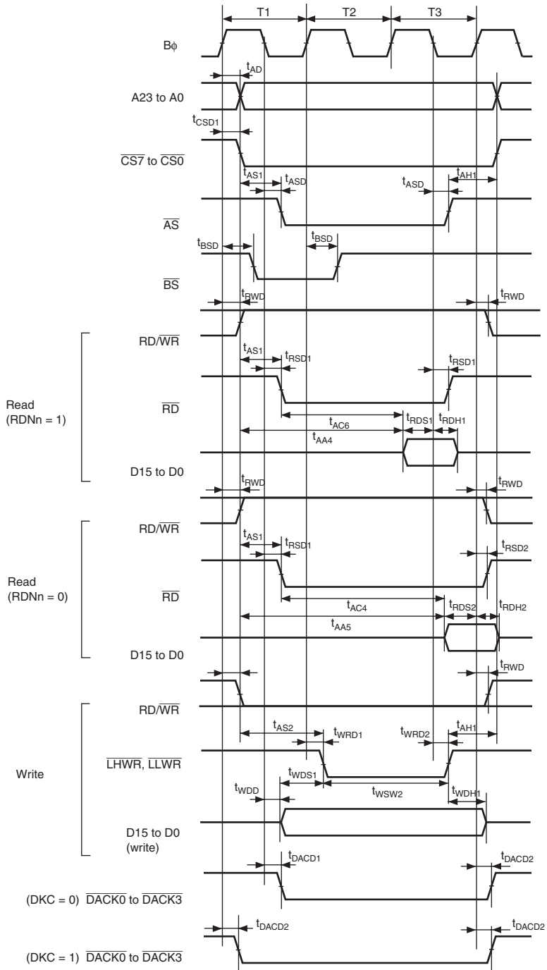
Figure 22.9 Basic Bus Timing: 3-State Access
