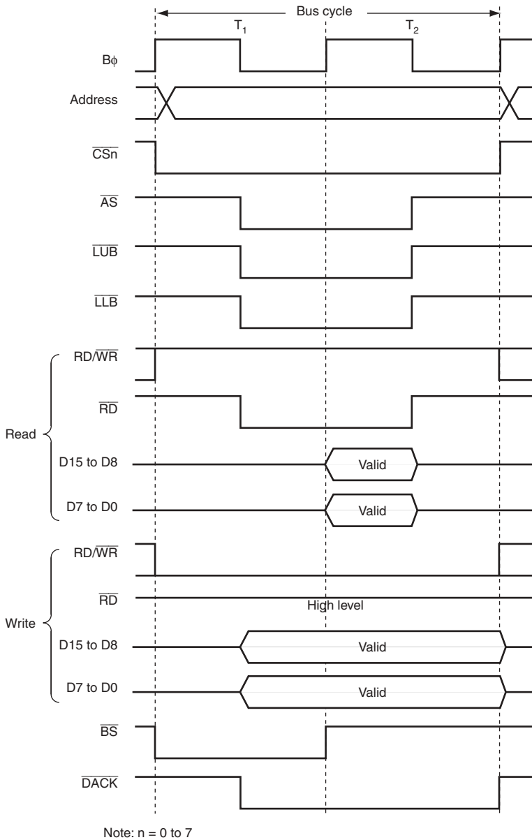
Figure 6.24 16-Bit 2-State Access Space Bus Timing
