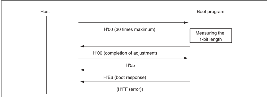
Figure 18.24 Bit-Rate-Adjustment Sequence
