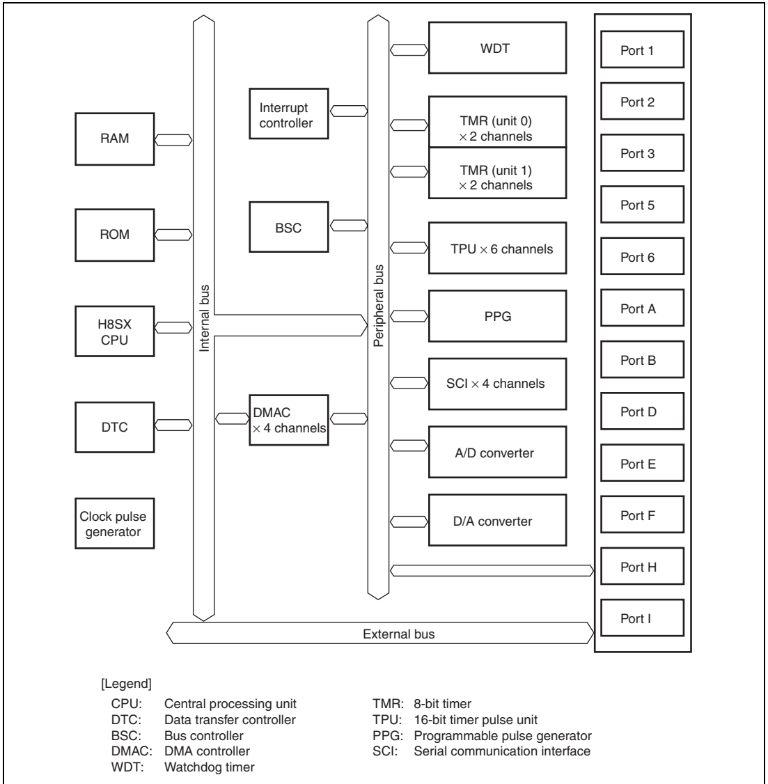
Figure 1.1 Block Diagram
