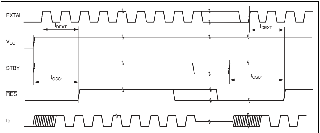
Figure 22.4 Oscillation Settling Timing
