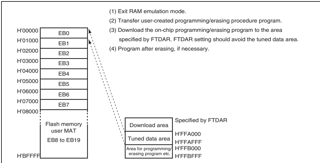
Figure 18.21 Programming Tuned Data
