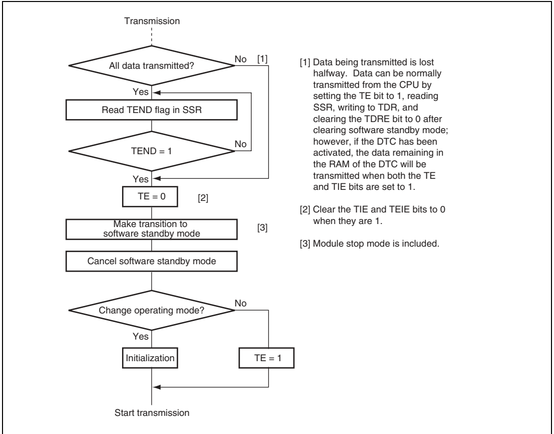
Figure 14.34 Sample Flowchart for Mode Transition during Transmission
