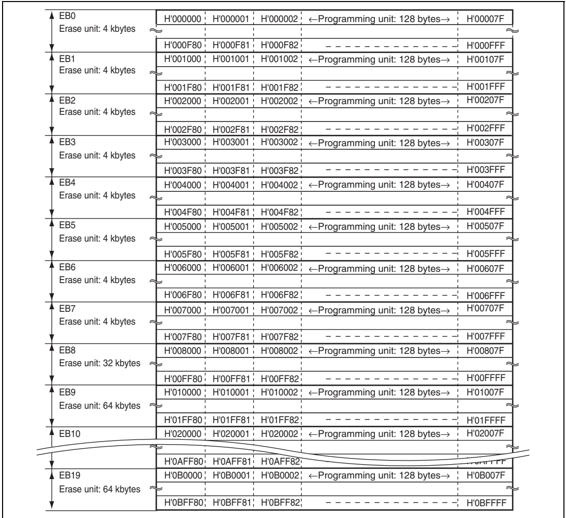
Figure 18.4 Block Structure of User MAT
