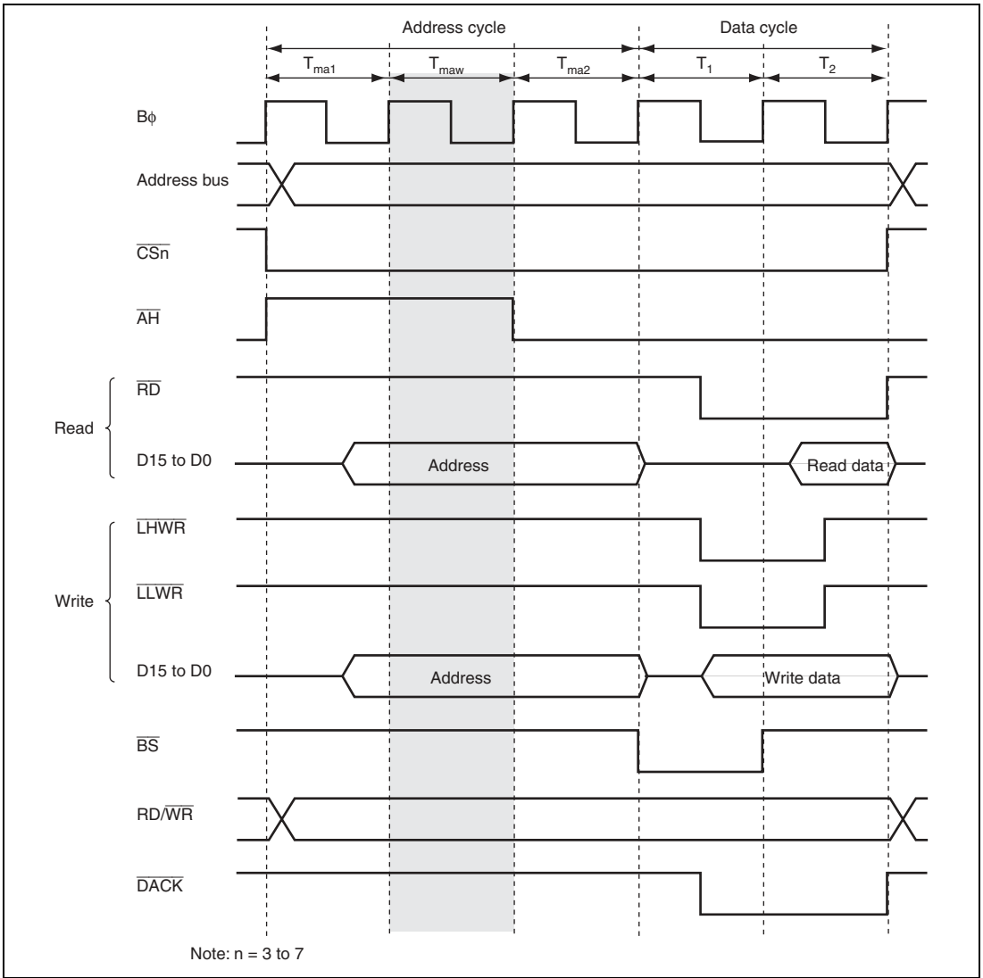
Figure 6.32 Access Timing of 3 Address Cycles (ADDEX = 1)
