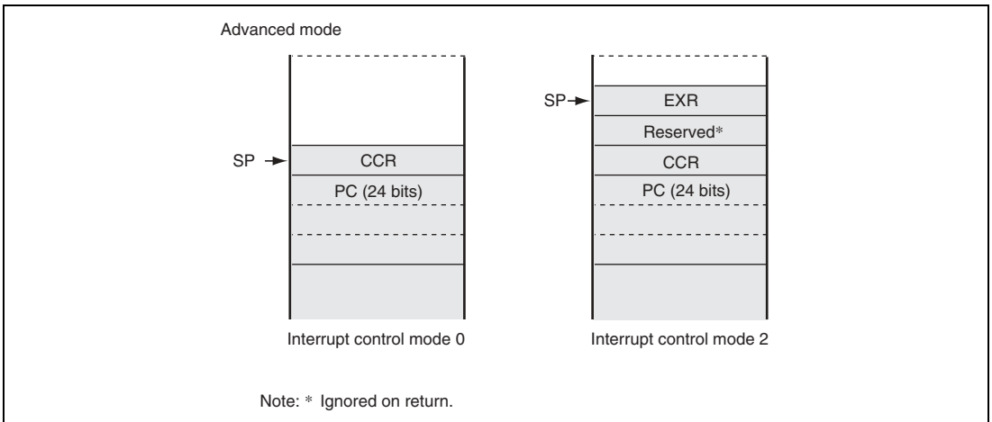
Figure 4.3 Stack Status after Exception Handling
