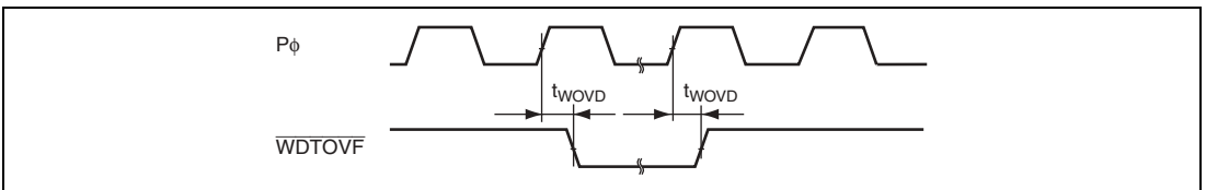
Figure 22.32 WDT Output Timing
