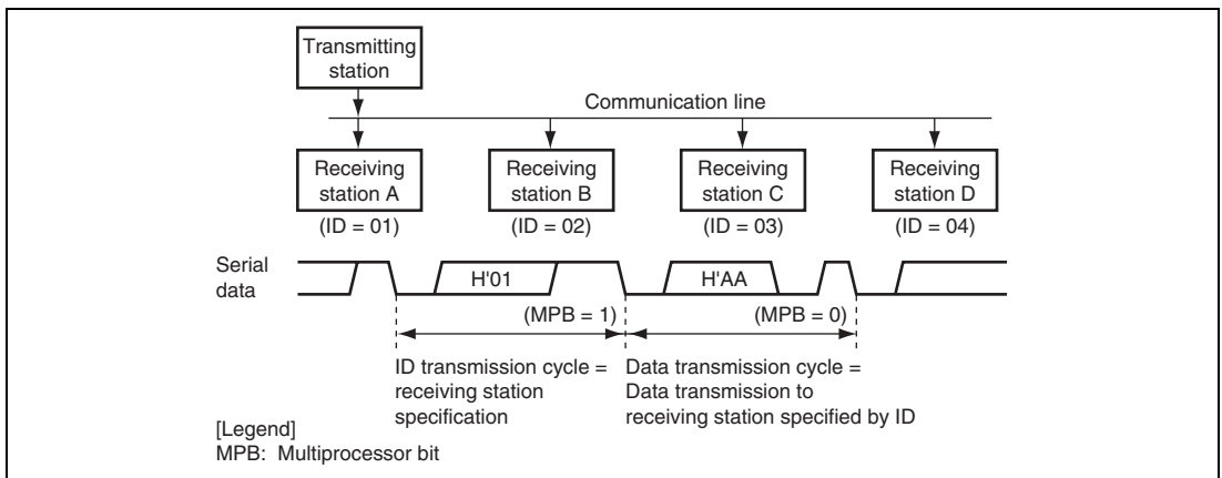
Figure 14.10 Example of Communication Using Multiprocessor Format (Transmission of Data H'AA to Receiving Station A)
