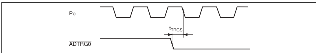
Figure 22.35 A/D Converter External Trigger Input Timing
