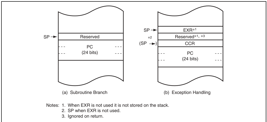
Figure 2.5 Stack Structure (Middle and Advanced Modes)
