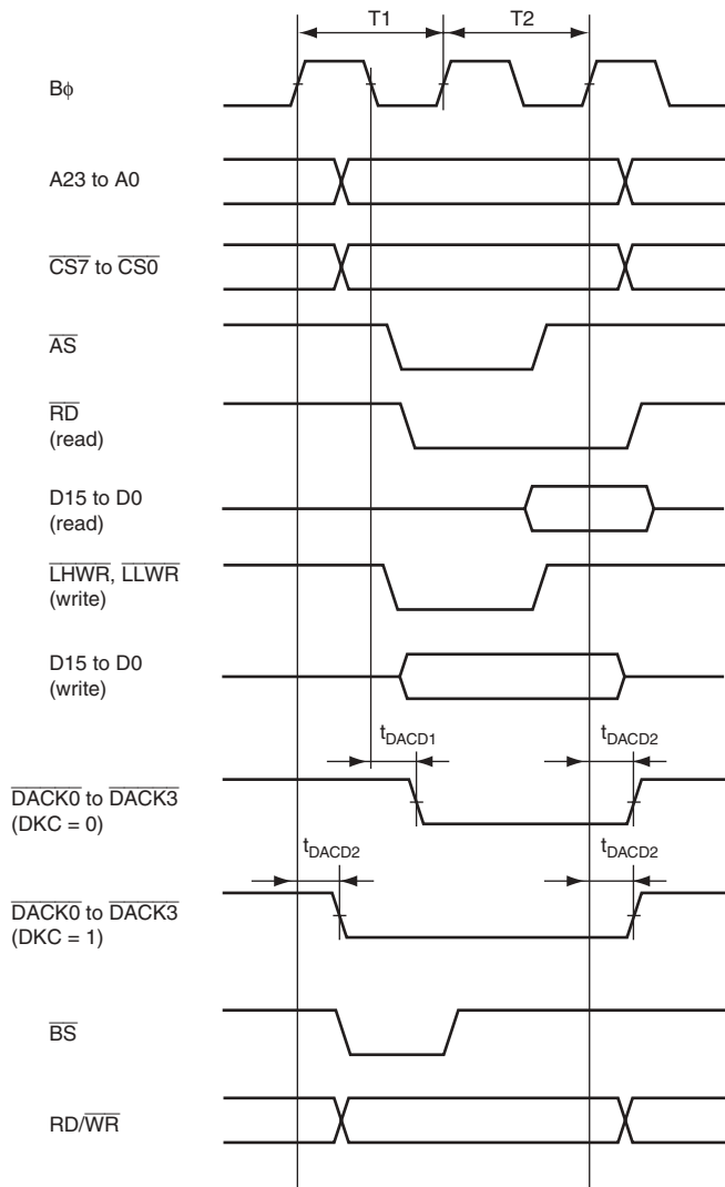
Figure 22.23 DMAC Single-Address Transfer Timing: 2-State Access
