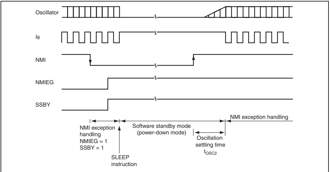
Figure 22.3 Oscillation Settling Timing after Software Standby Mode
