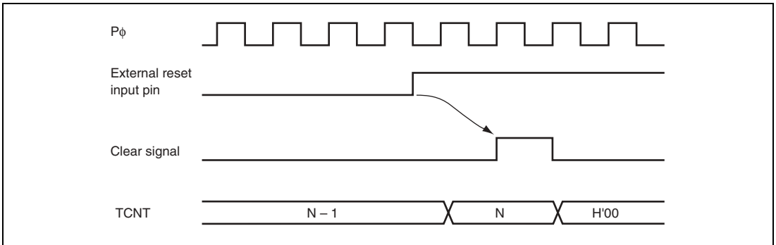
Figure 12.10 Timing of Clearance by External Reset (Rising Edge)
