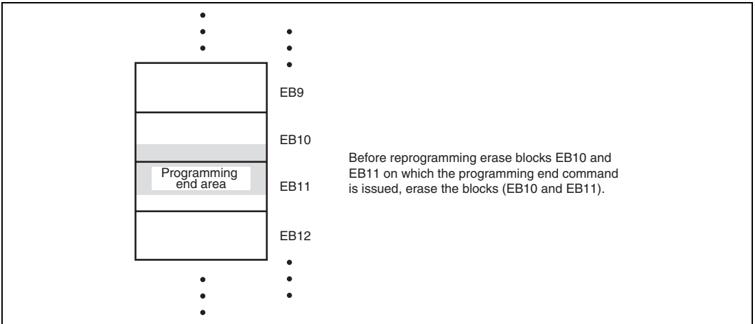
Figure 18.13 Example of Erase Block Including Programmed Area
