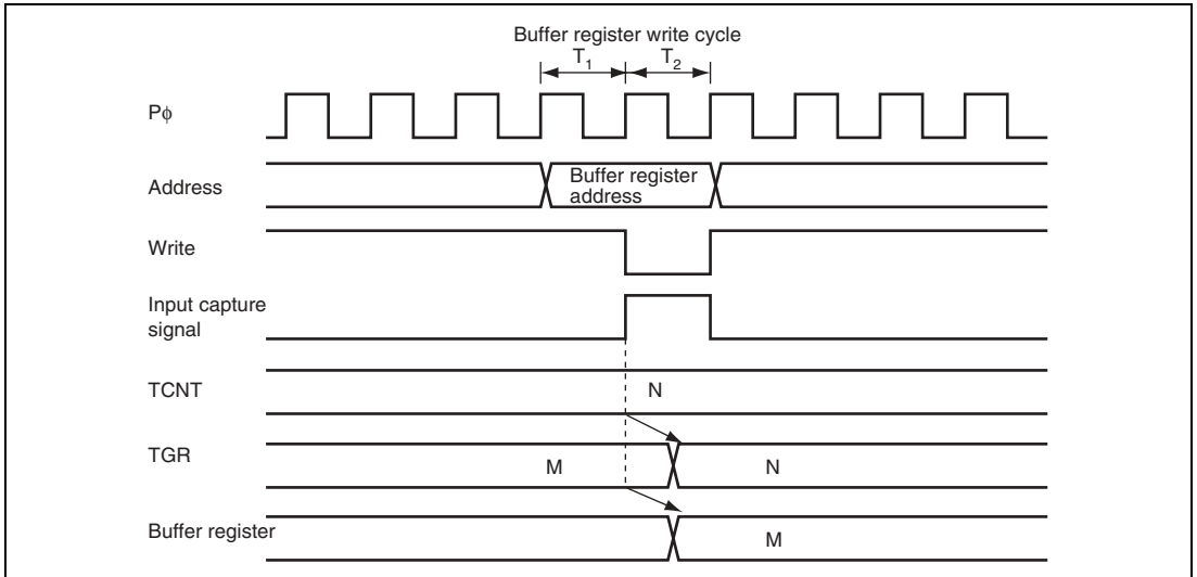
Figure 10.52 Conflict between Buffer Register Write and Input Capture
