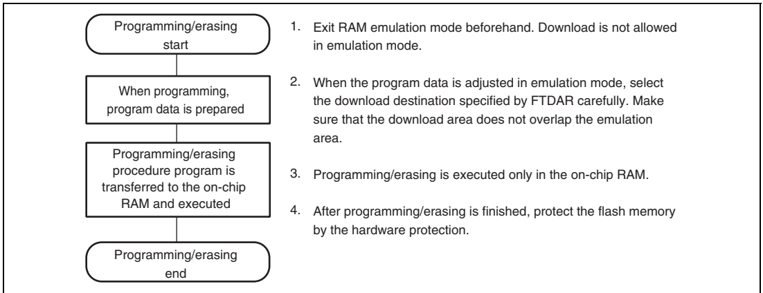
Figure 18.10 Programming/Erasing Flow
