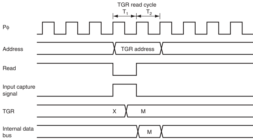
Figure 10.50 Conflict between TGR Read and Input Capture
