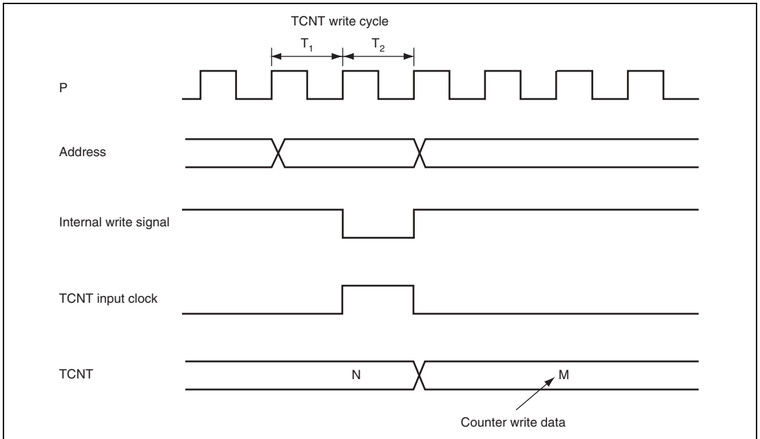
Figure 13.5 Conflict between TCNT Write and Increment
