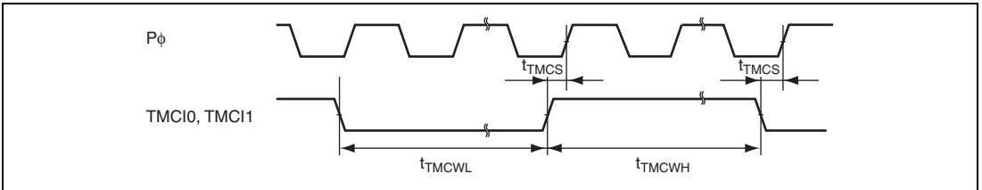
Figure 22.31 8-Bit Timer Clock Input Timing
