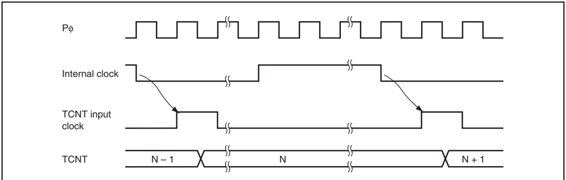
Figure 12.5 Count Timing for Internal Clock Input (Falling Edge)
