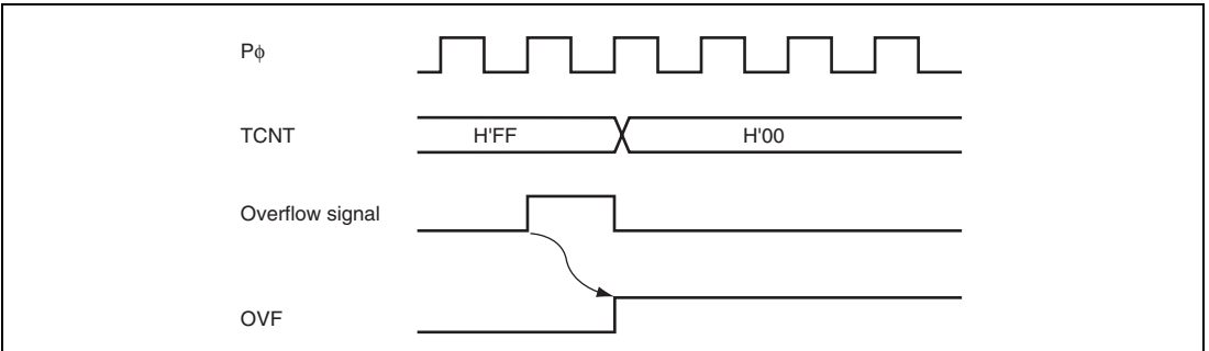
Figure 12.12 Timing of OVF Setting
