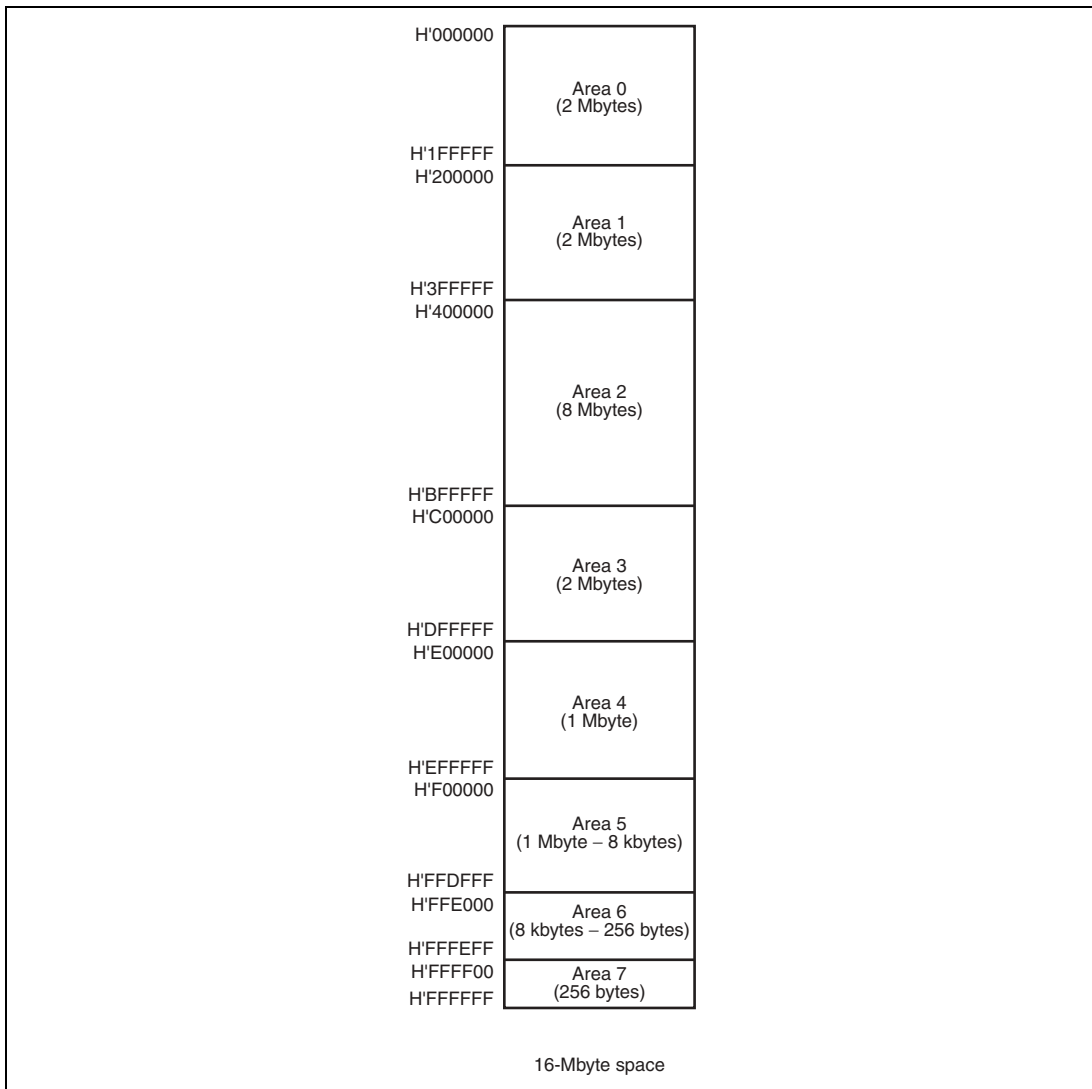
Figure 6.7 Address Space Area Division
