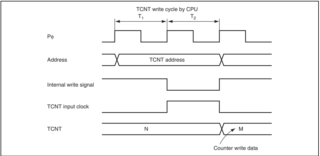
Figure 12.14 Conflict between TCNT Write and Increment
