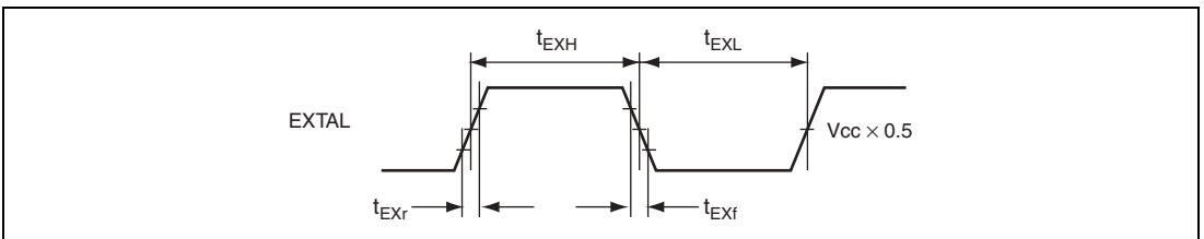
Figure 22.5 External Input Clock Timing
