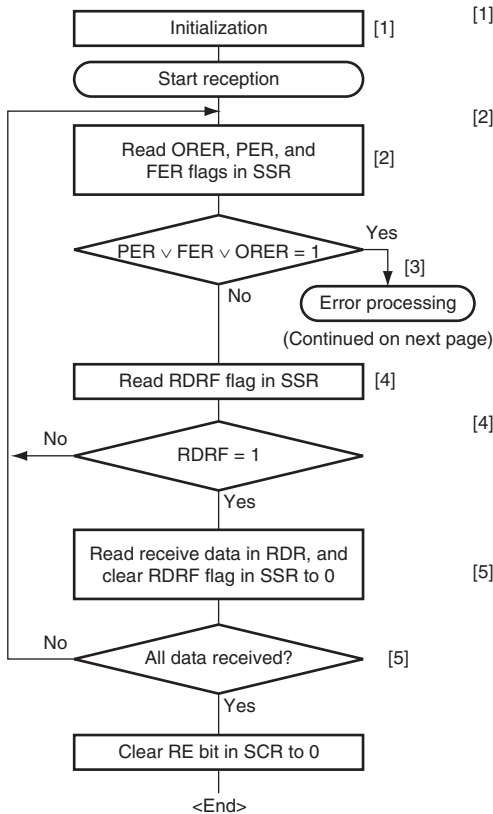
Figure 14.9 Sample Serial Reception Flowchart (1)
