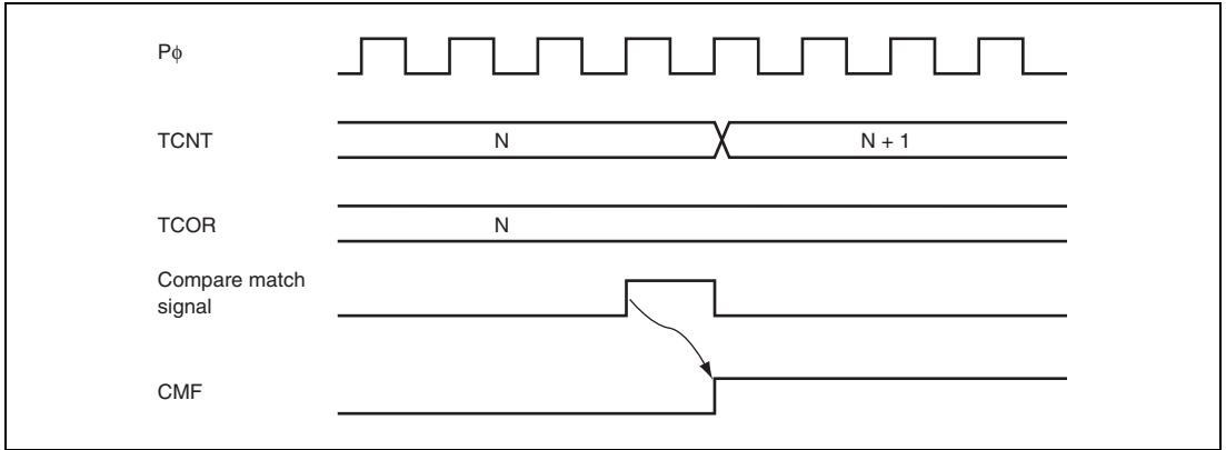
Figure 12.7 Timing of CMF Setting at Compare Match
