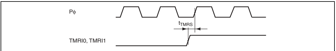
Figure 22.30 8-Bit Timer Reset Input Timing
