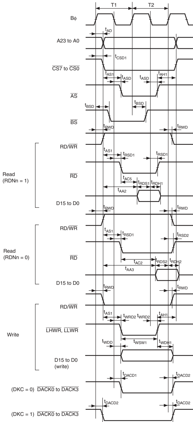
Figure 22.8 Basic Bus Timing: 2-State Access
