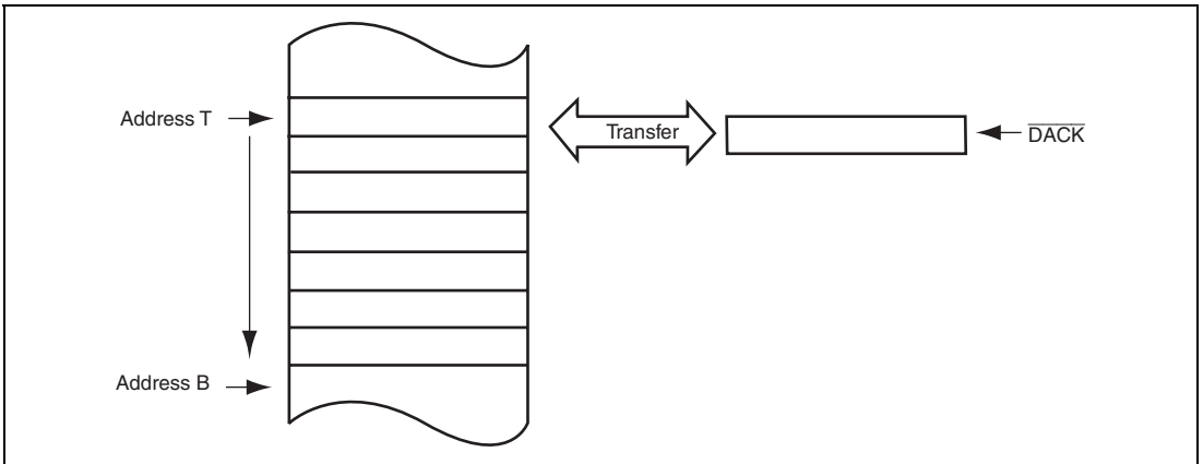
Figure 7.6 Operations in Single Address Mode
