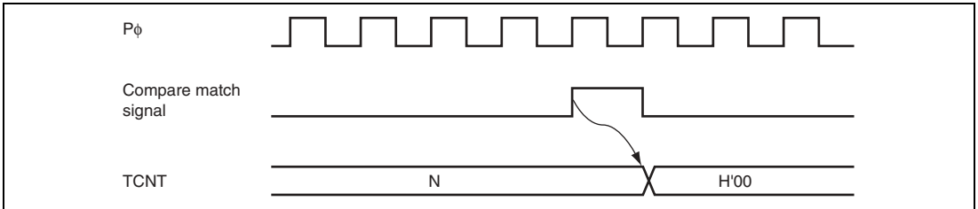
Figure 12.9 Timing of Counter Clear by Compare Match
