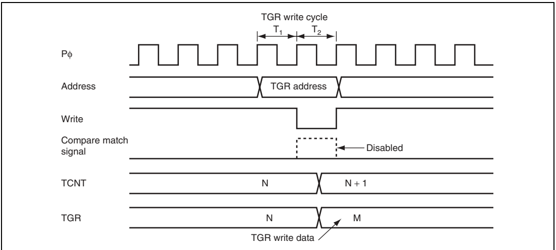
Figure 10.48 Conflict between TGR Write and Compare Match
