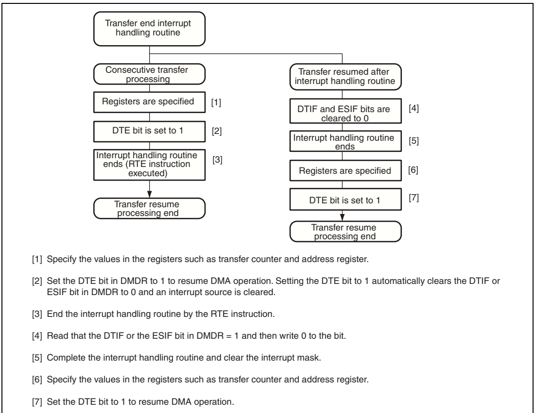
Figure 7.40 Procedure Example of Resuming Transfer by Clearing Interrupt Source
