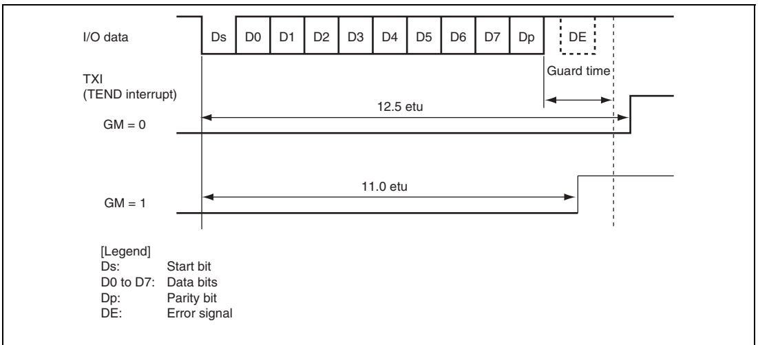
Figure 14.27 TEND Flag Set Timing during Transmission
