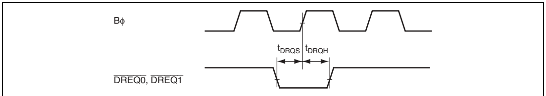
Figure 22.21 DMAC ( \overline{\text{DREQ}} ) Input Timing
