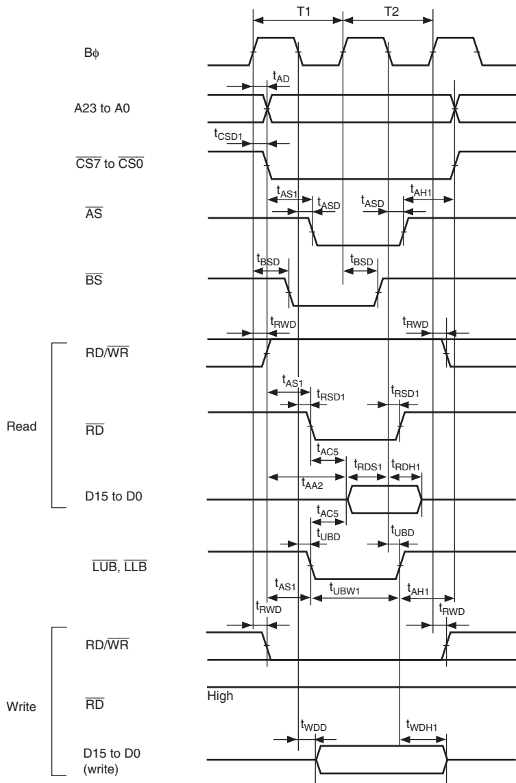
Figure 22.13 Byte Control SRAM: 2-State Read/Write Access
