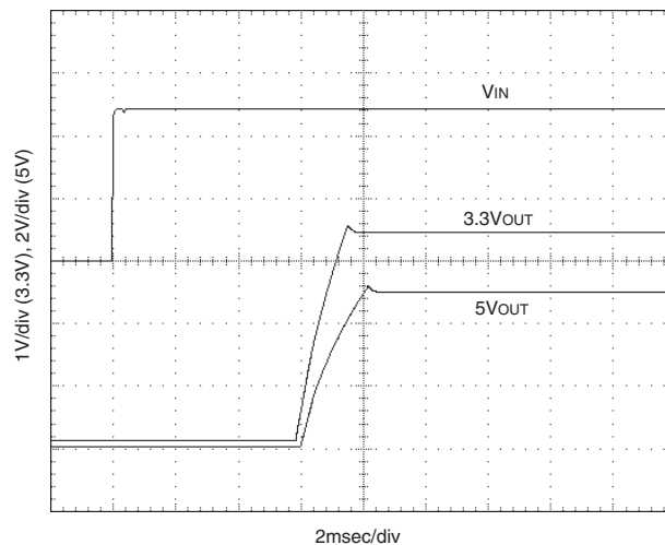
(V IN = nominal, 5V @ 1.5A/3.3V @ 2.25A, 0.47μF || 100μF tantalum output capacitors.)
