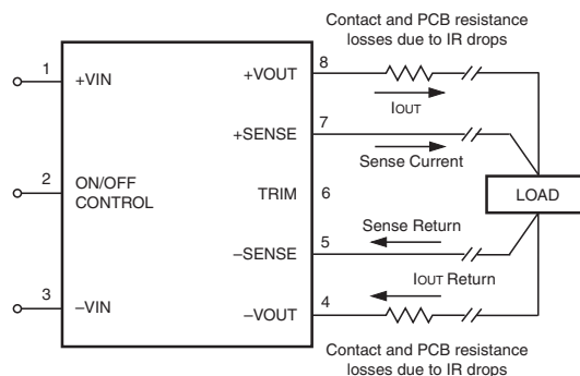
Figure 8. Remote Sense Circuit Configuration
