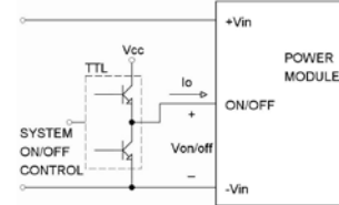
Level Control Using TTL Output
