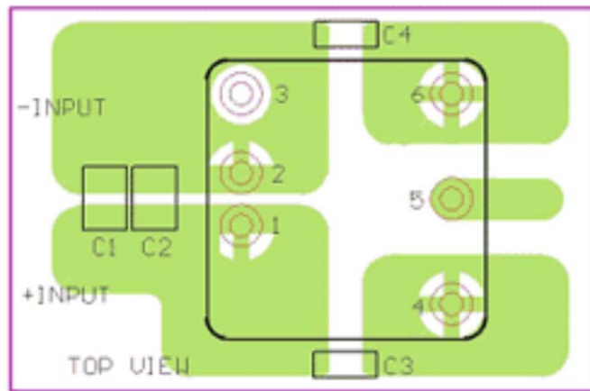
Recommended layout with input filter
