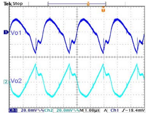
Typical Output Ripple and Noise. V_{in,nom} ; Full Load
