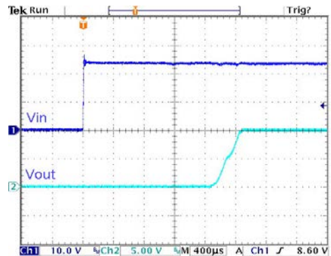
Typical Input Start-Up and Output Rise Characteristic V_{in,nom} ; Full Load
