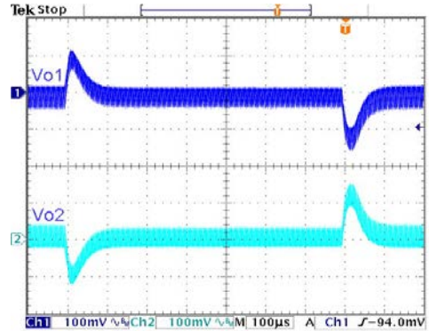
Transient Response to Dynamic Load Change from 100% to 75% to 100% of Full Load ; V_{in,nom}
