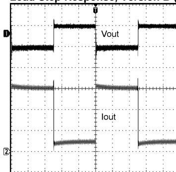
Load Step Response, Version B (4.5V)
