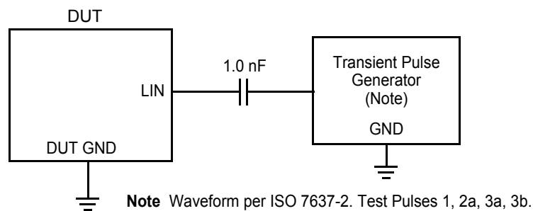
Figure 6. Test Circuit for Transient Test Pulses (LIN)
