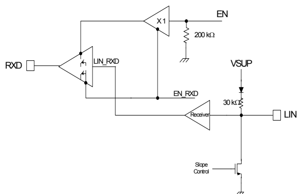
Figure 28. RXD Interface
