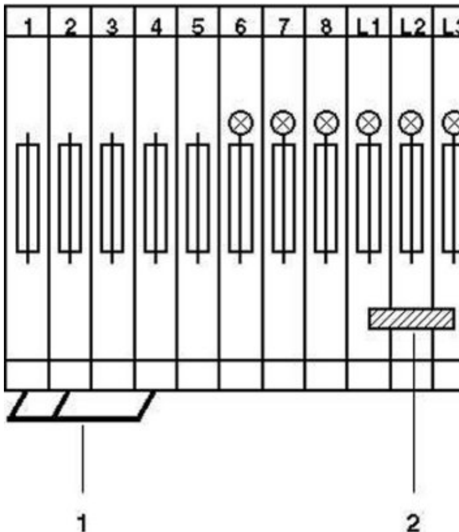
Circuit diagram
