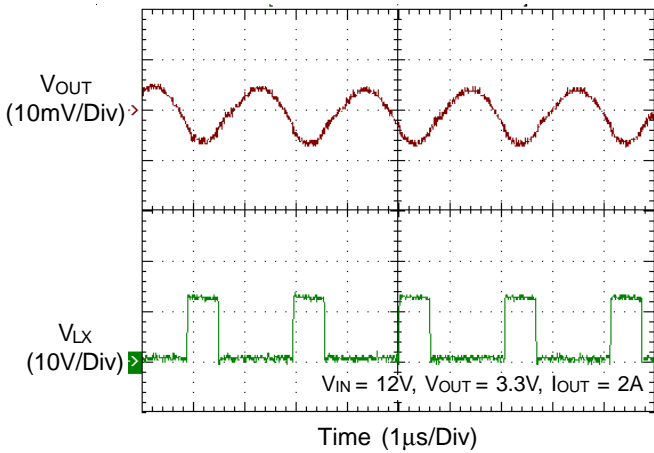
Voltage Ripple
