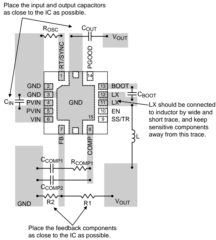
Figure 11. PCB Layout Guide
