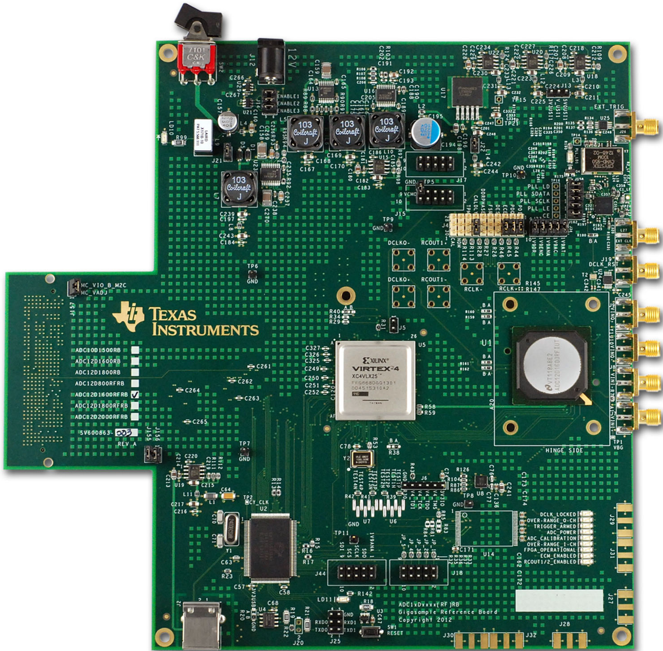
Figure 2. ADC1xDxxx(RF)RB Board Layout
