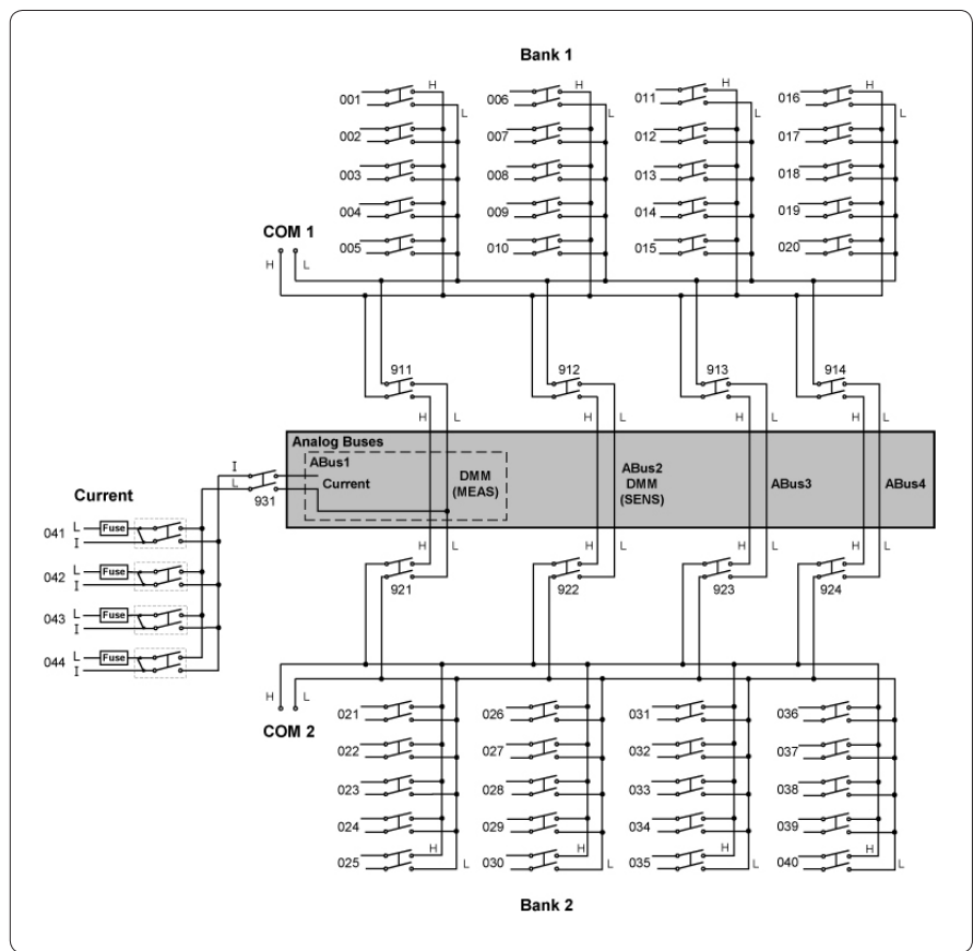
Figure 1. L4421A 40-channel armature multiplexer with low thermal offset (bank 2).
