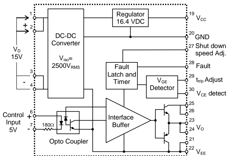
Figure 1: VLA500 Series Block Diagram
