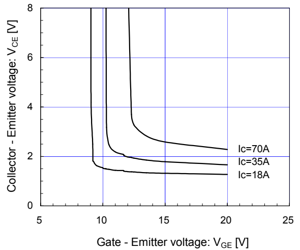
[ Brake ] Collector-Emitter voltage vs. Gate-Emitter voltage (typ.) T_j = 25^\circ\text{C} / \text{chip}
