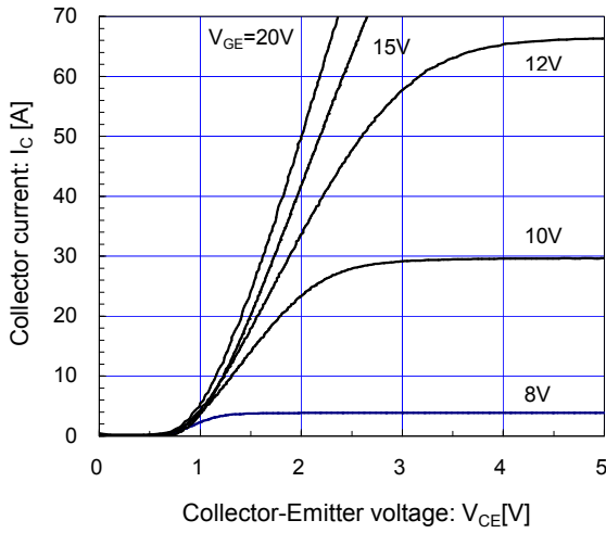
[ Brake ] Collector current vs. Collector-Emitter voltage (typ.) T_j = 25^\circ\text{C} / \text{chip}
