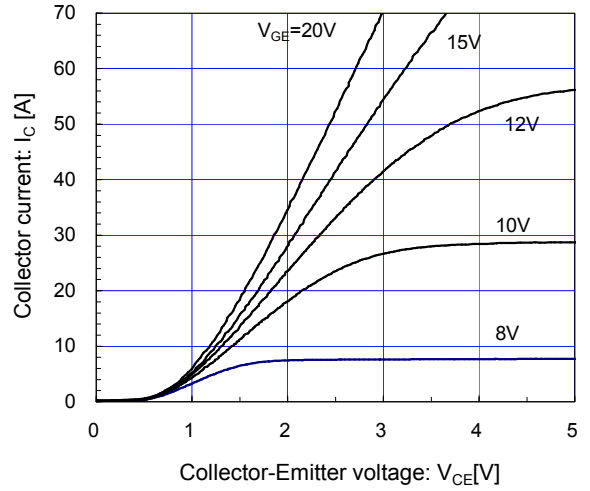
[ Brake ] Collector current vs. Collector-Emitter voltage (typ.) T_j = 150^\circ\text{C} / \text{chip}
