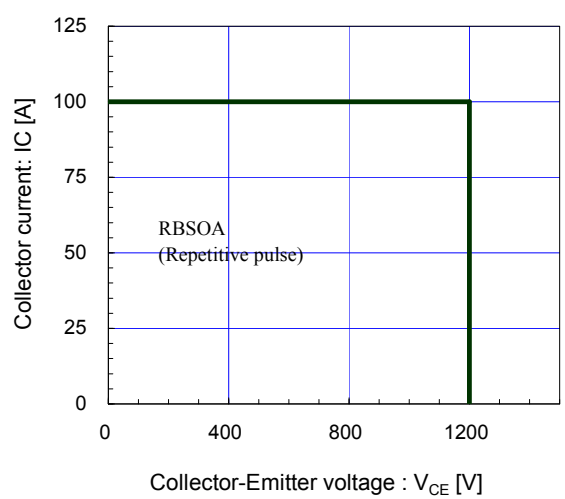
[ Inverter ] Reverse bias safe operating area (max.) +V_{GE}=15V, -V_{GE} \le 15V, R_g \ge 15\Omega, T_j=150^\circ C
