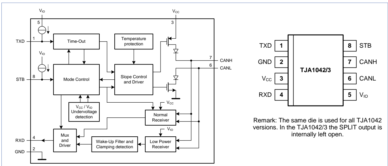
Fig 21. Block diagram and pinning of the TJA1042/3
