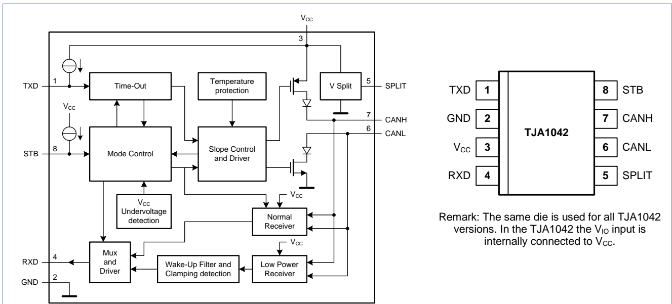
Fig 20. Block diagram and pinning of the TJA1042
