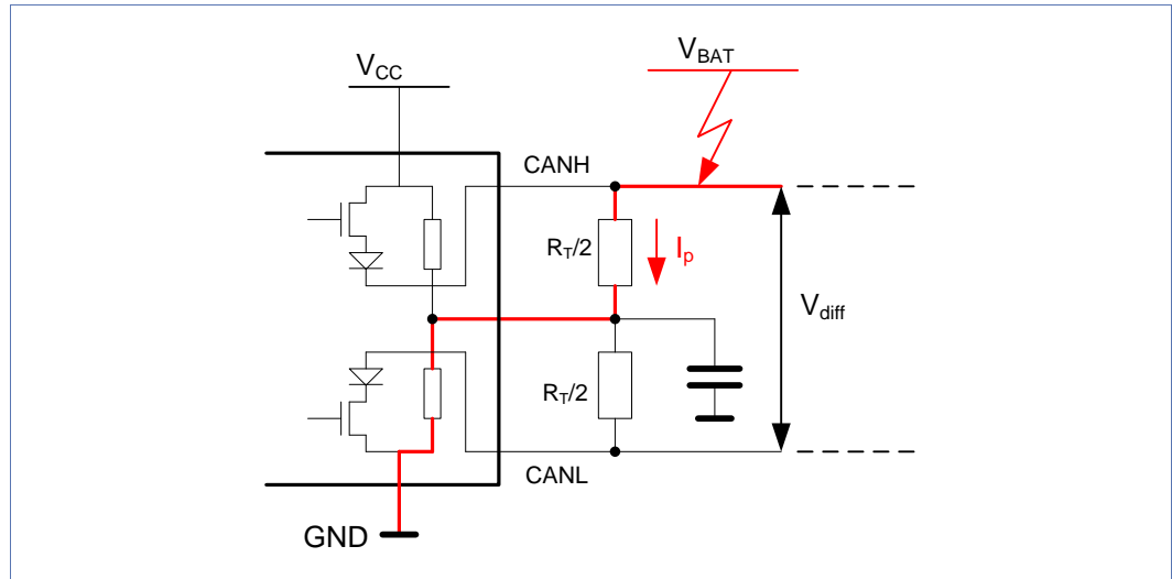
Fig 38. Bus dominant clamping in the case of a short circuit CANH to V_{BAT}
