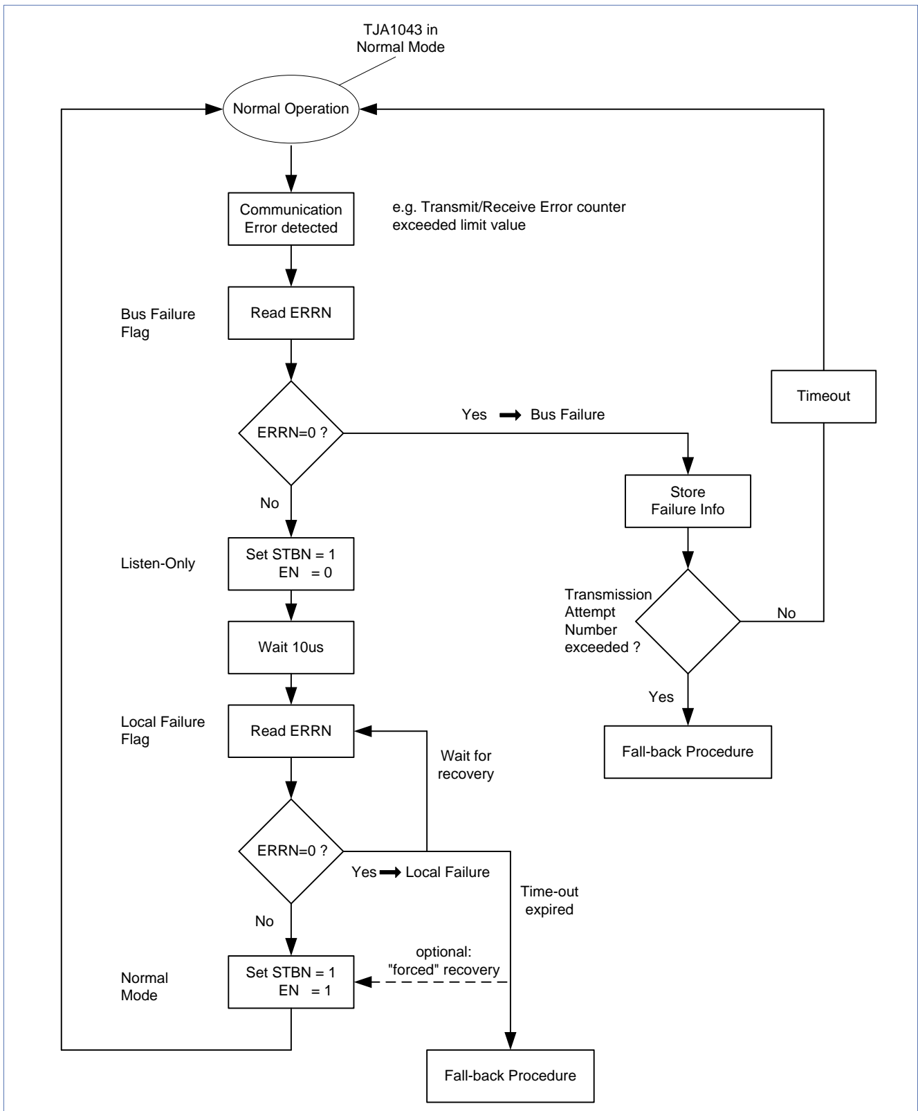
Fig 39. Flow diagram for handling communication failures
