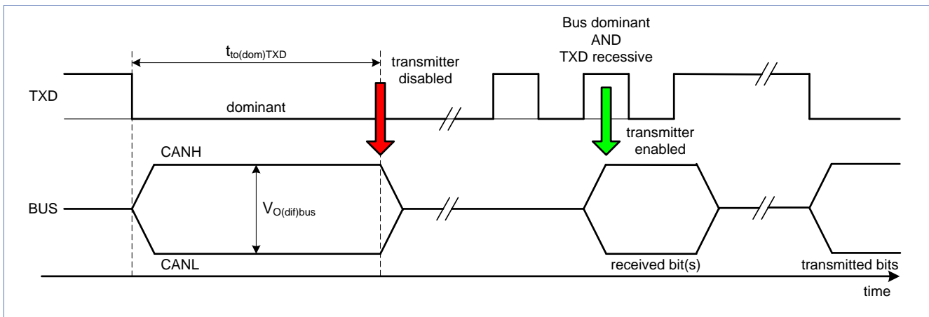
Fig 37. TXD dominant timeout and recovery mechanism
