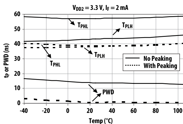
Figure 17. Improvement of t_p and PWD with added 100pF peaking capacitor in parallel of input limiting resistor.
