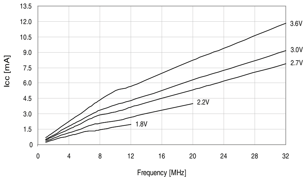
Figure 37-257. Active supply current vs. frequency.
