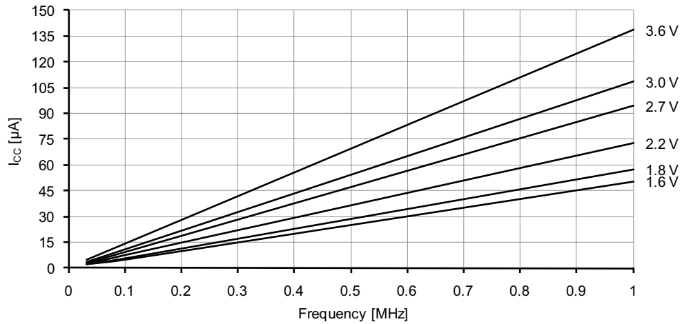
Figure 37-178. Idle mode supply current vs. frequency.
