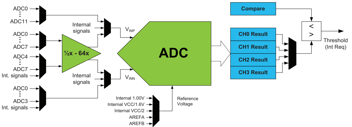
Figure 28-1. ADC overview.
