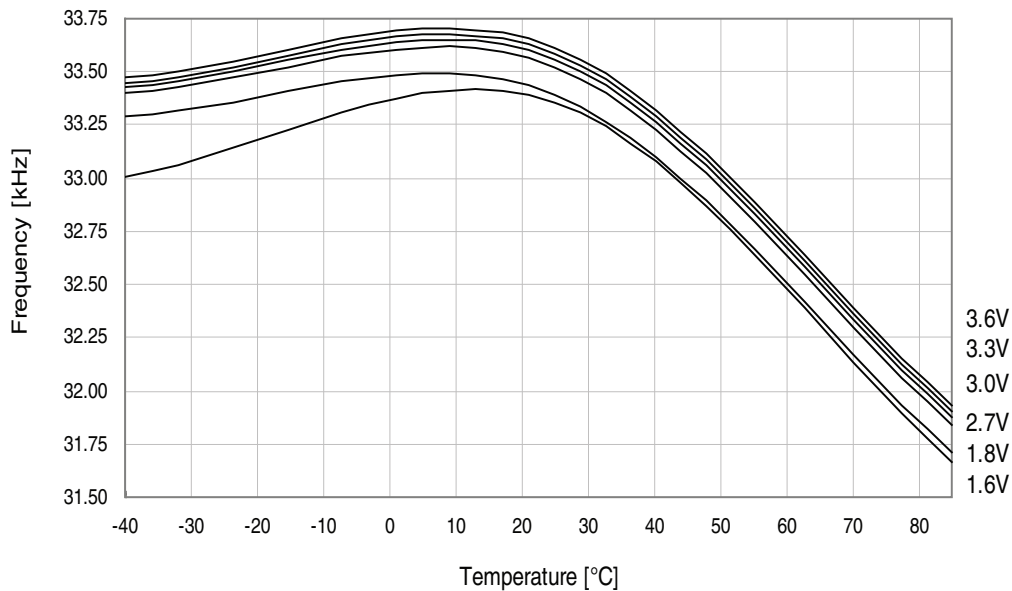
Figure 37-325. Ultra Low-Power internal oscillator frequency vs. temperature.
