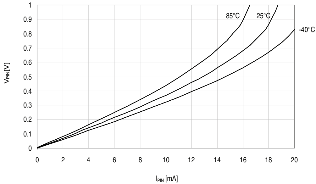
Figure 37-283. I/O pin output voltage vs. sink current.
