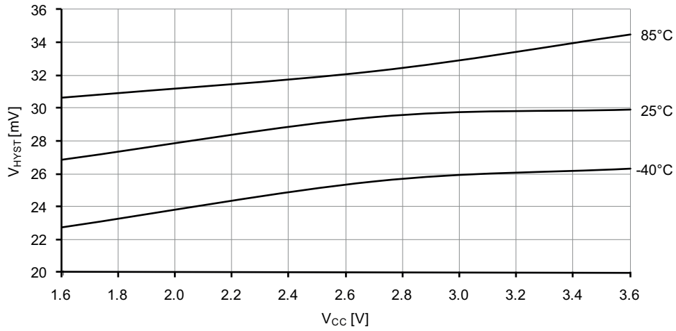
Figure 37-224. Analog comparator hysteresis vs. V_{CC} .
