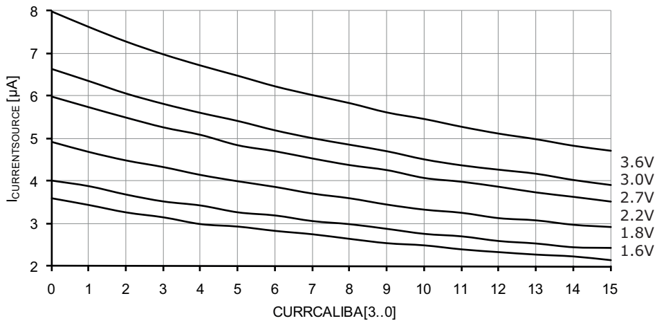
Figure 37-226. Analog comparator current source vs. calibration value.
