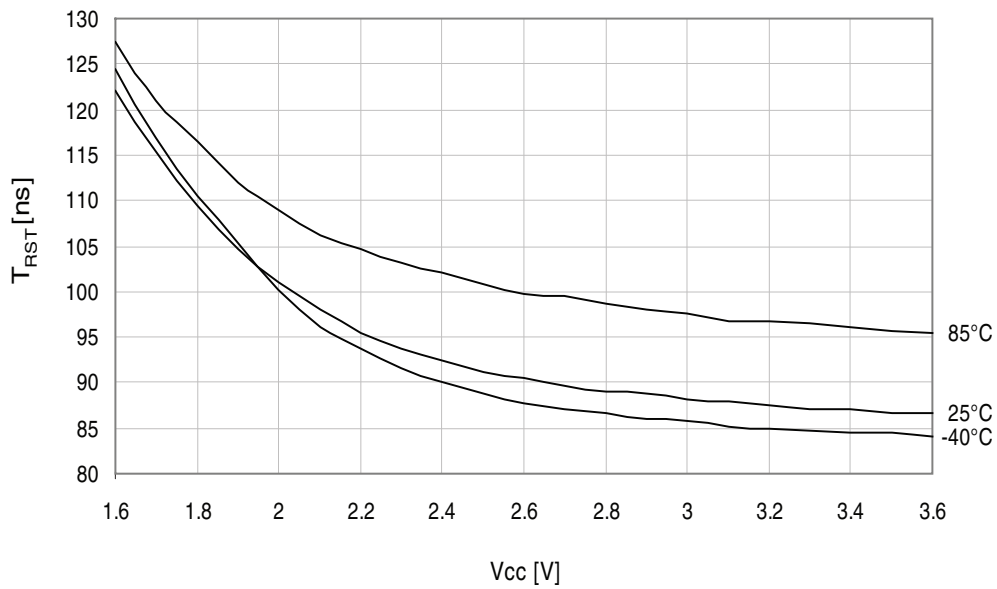
Figure 37-317. Minimum Reset pin pulse width vs. V CC .
