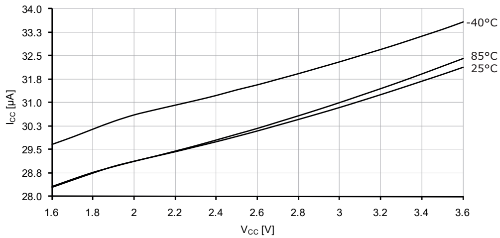
Figure 37-180. Idle mode supply current vs. V_{CC} .
