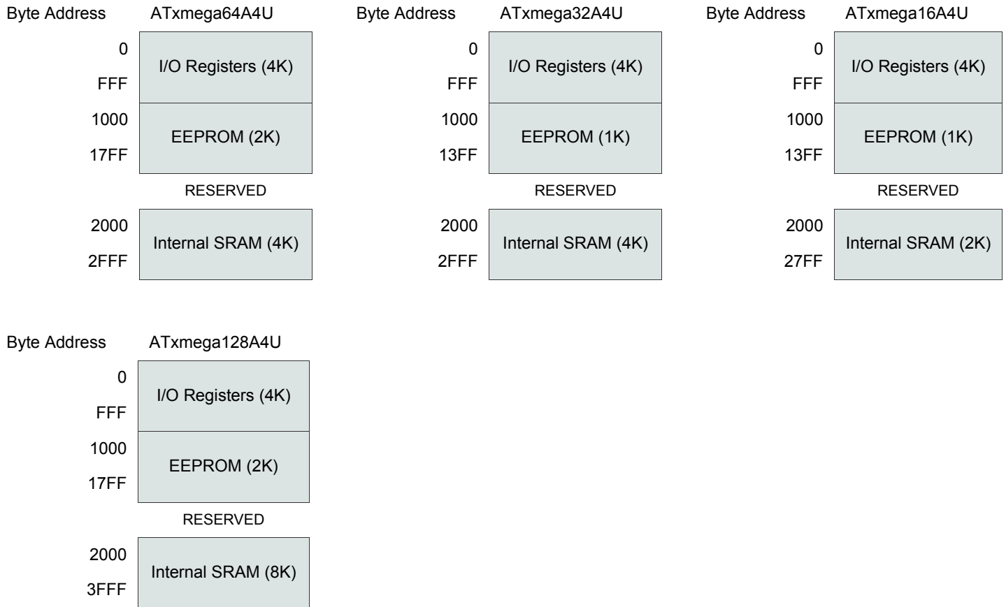
Figure 7-3. Data memory map (Hexadecimal address).
