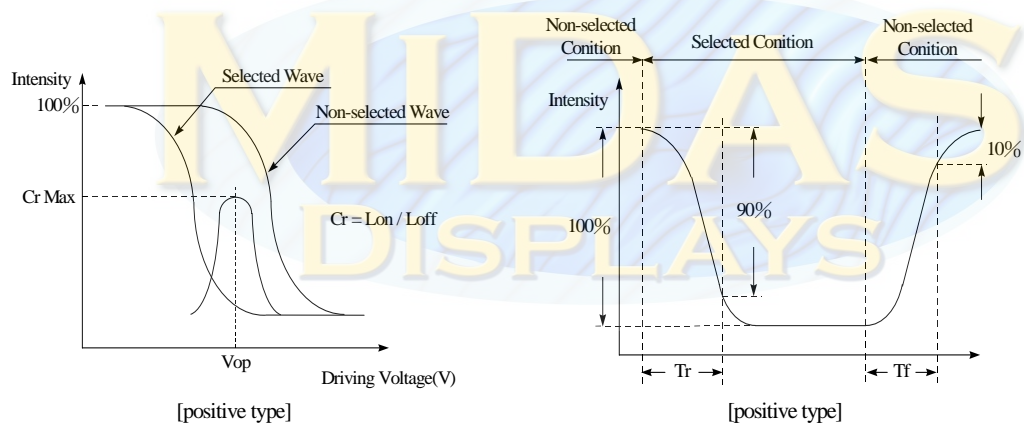
Definition of Operation Voltage (Vop)
