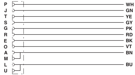
Contact assignment of the M16 socket
