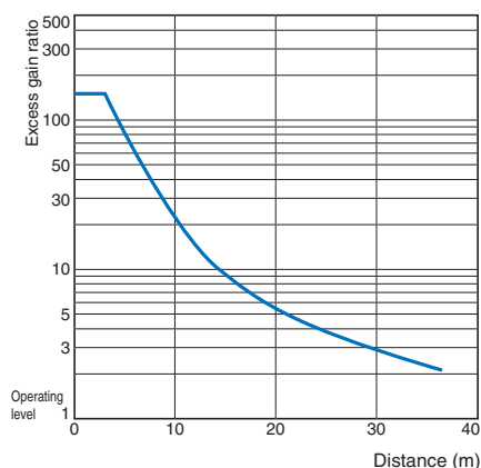
Through-beam E3S-CT□1 (-M1J)
