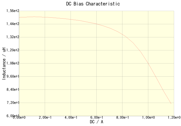
SLF7045T-151MR50-H(Amb. Temp. = 20degc)
