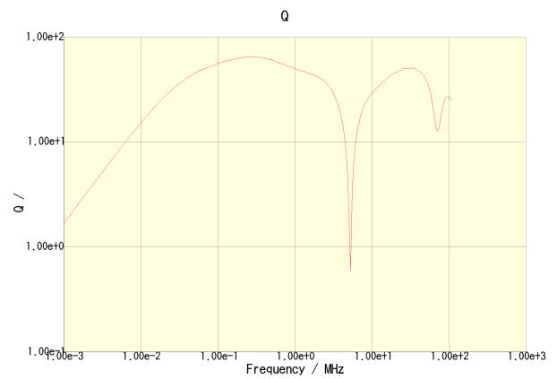
SLF7045T-151MR50-H
