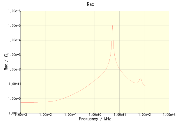
SLF7045T-151MR50-H
