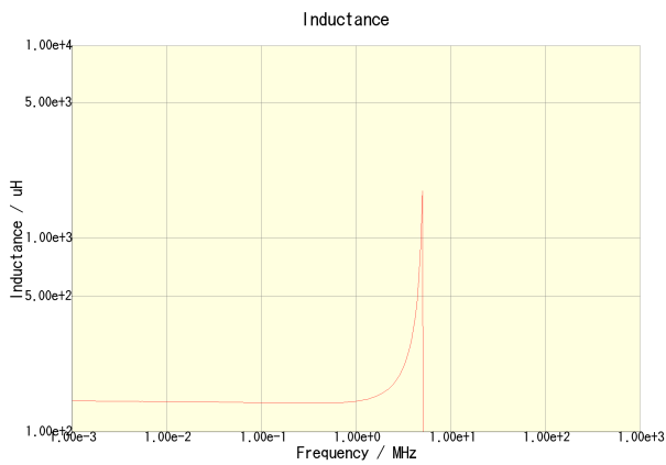
SLF7045T-151MR50-H
