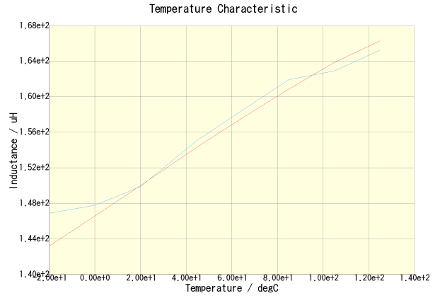
SLF7045T-151MR50-H(DC = 0A)
