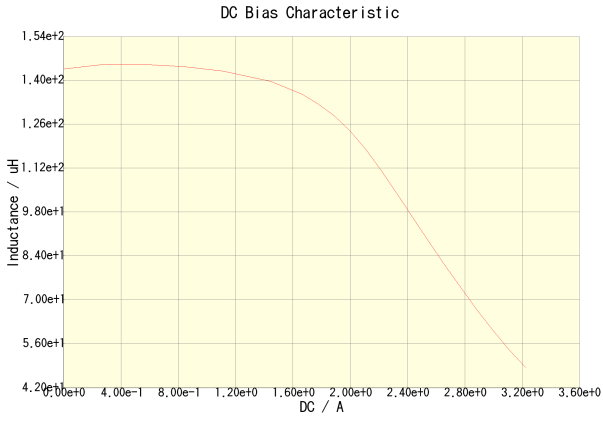
SLF12575T-151M1R5-H(Amb. Temp. = 20degc)
