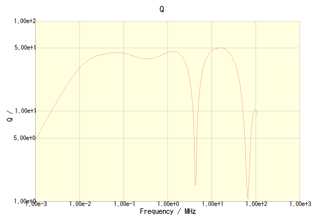
SLF12575T-151M1R5-H
