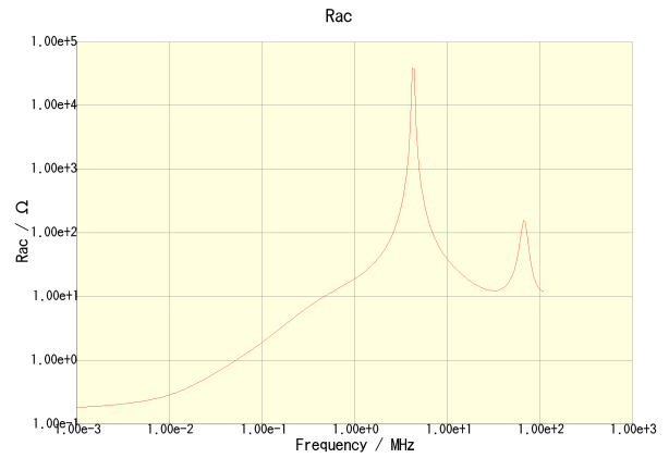
SLF12575T-151M1R5-H
