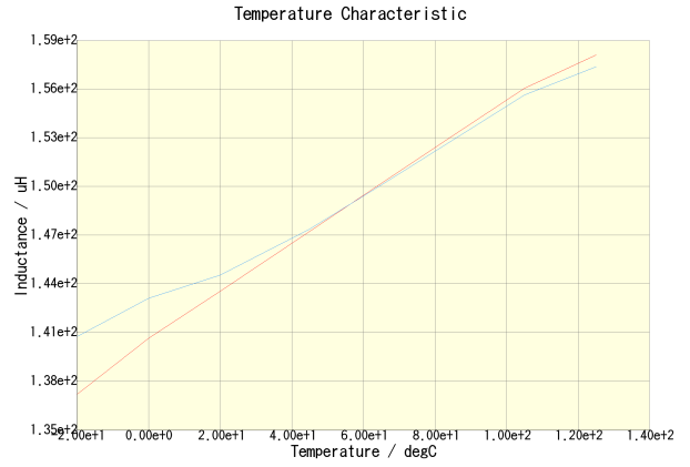
SLF12575T-151M1R5-H(DC = 0A) SLF12575T-151M1R5-H(DC = 0.75A)
