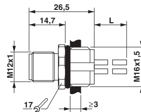
Dimensioned drawing
