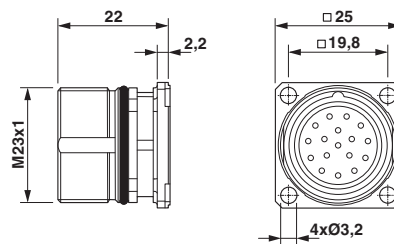
Dimensioned drawing
