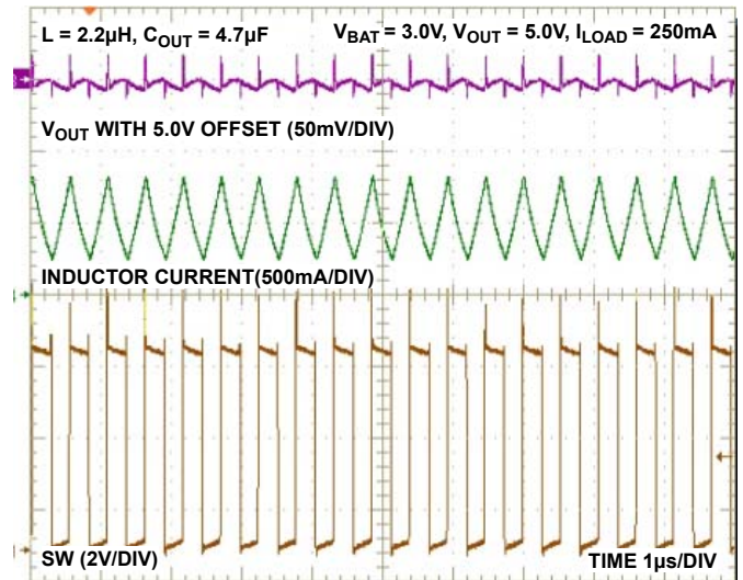
FIGURE 7. PWM WAVEFORM
