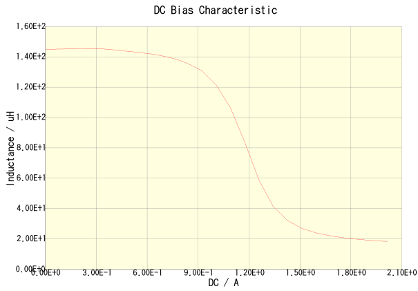
SLF10145T-151MR79-PF(Amb. Temp. = 20degc)
