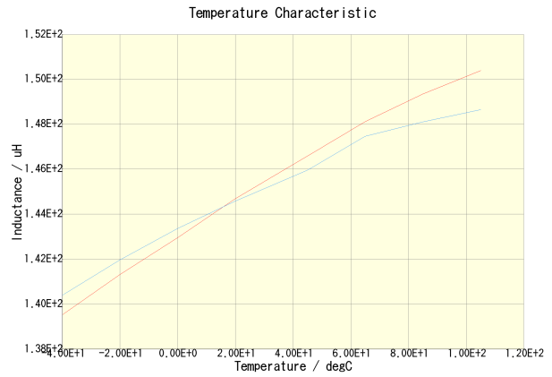
SLF10145T-151MR79-PF(DC = 0A) SLF10145T-151MR79-PF(DC = 0.395A)
