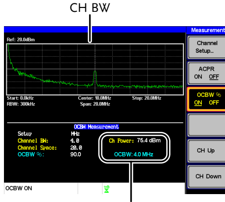
Channel power and OCBW power results
