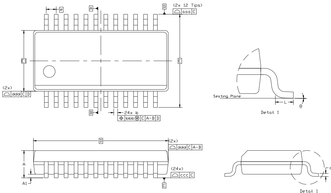
Figure 6.1. QSOP-24 Package Drawing
