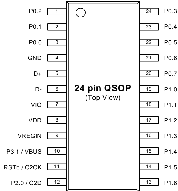
Figure 4.2. EFM8UB1xFxxG-A-QSOP24 Pinout
