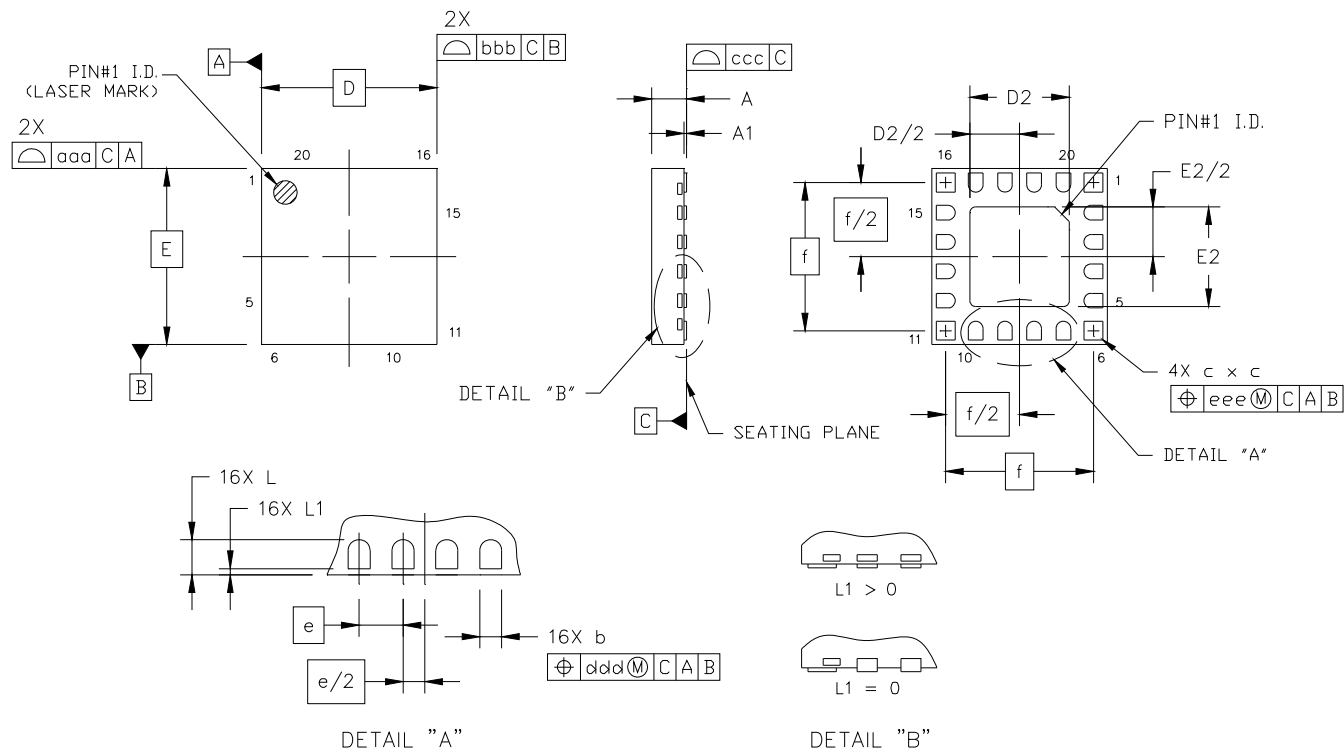
Figure 7.1. QFN-20 Package Drawing
