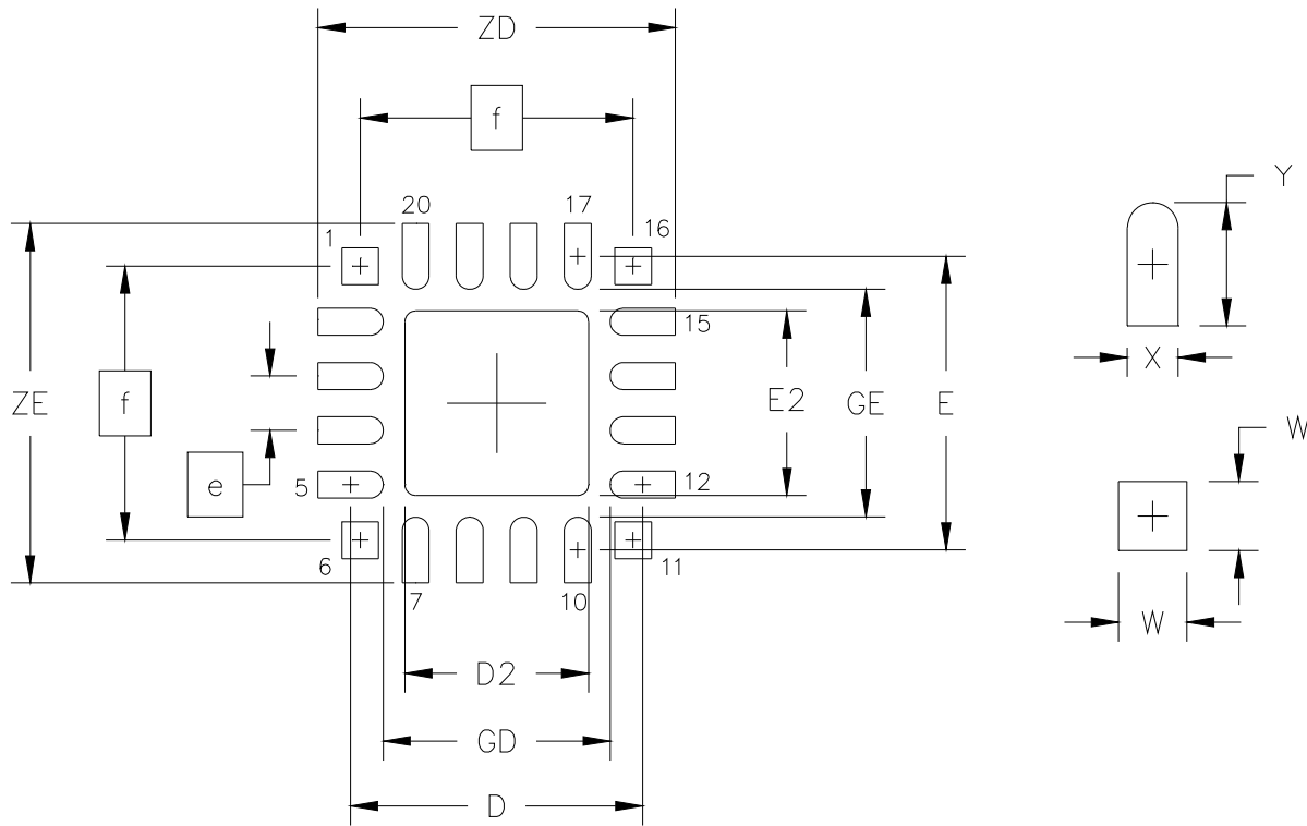
Figure 7.2. QFN-20 Landing Diagram
