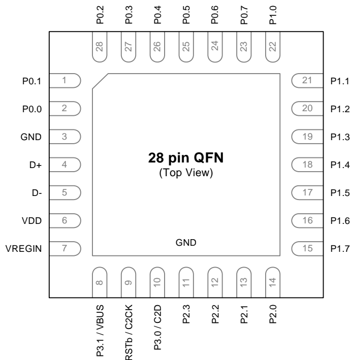
Figure 4.1. EFM8UB1xFxxG-A-QFN28 Pinout
