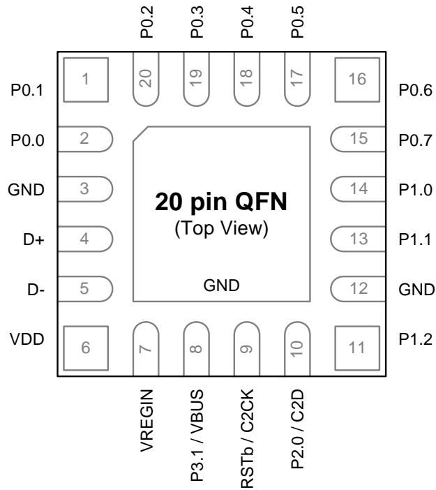
Figure 4.3. EFM8UB1xFxxG-A-QFN20 Pinout
