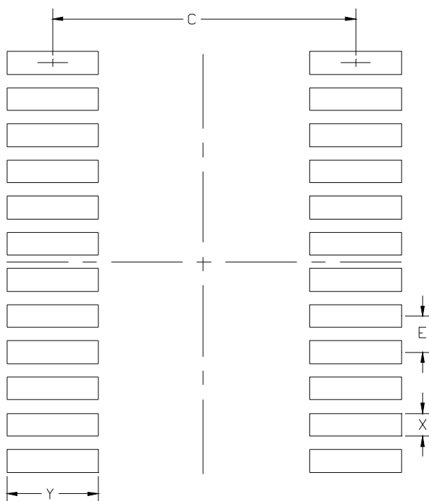
Figure 6.2. QSOP-24 PCB Land Pattern
