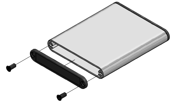
EXPLODED ASSEMBLY VIEW
