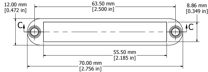
CLOSED BEZEL
