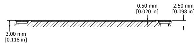
SECTION C-C
