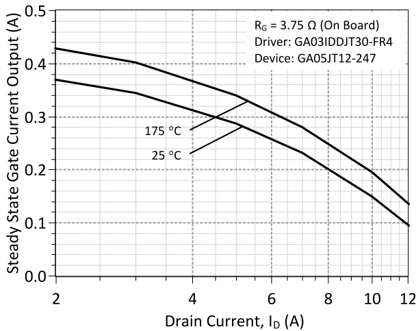
Figure 25: Typical steady state gate current supplied by the GA03IDDJT30-FR4 board for the GA05JT12-247 with the on board resistance of 3.75 Ω
