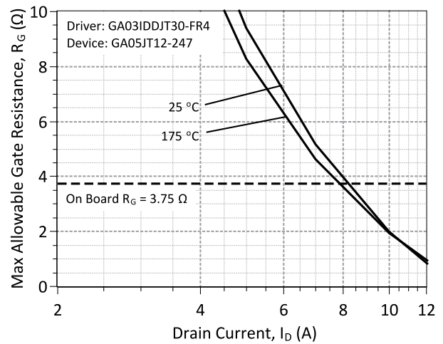
Figure 26: Maximum gate resistance for safe operation of the GA05JT12-247 at different drain currents using the GA03IDDJT30-FR4 board.
