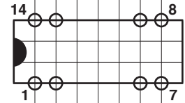
Circuit board pin spacing viewed from component side
