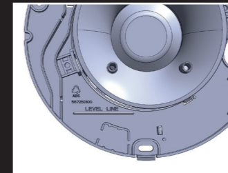
Radial fixing points and level reference line
