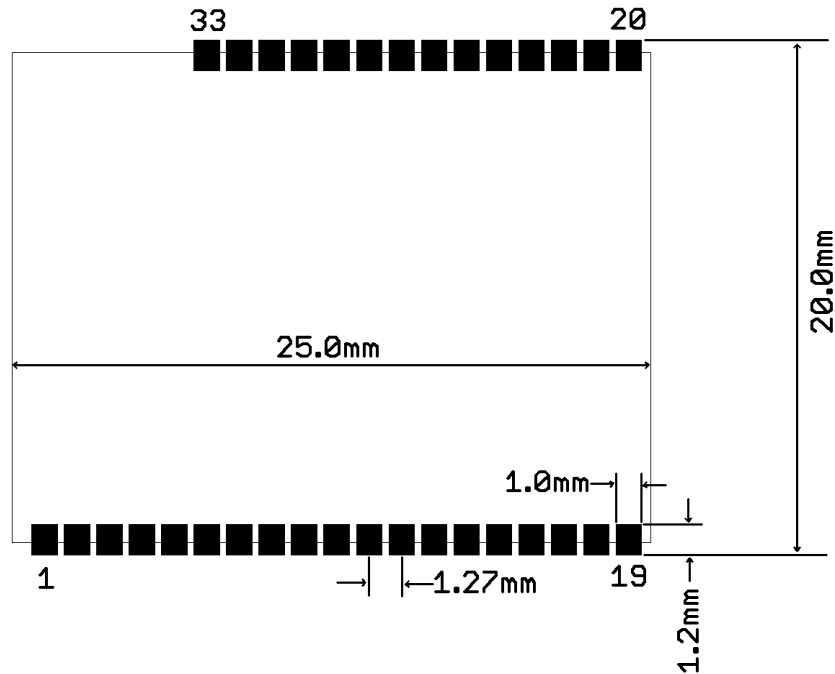
Figure 9: Recommended Footprint
