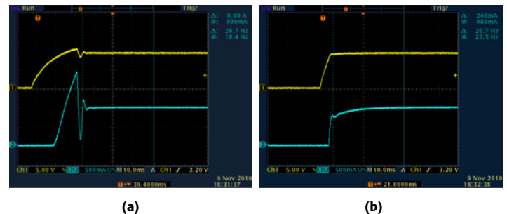
Figure 2. LED turn on voltage (yellow) and current (blue) waveforms when powered by a power supply in the traditional constant voltage (CV) mode (Figure 2a) and the constant current (CC) mode (Figure 2b).
