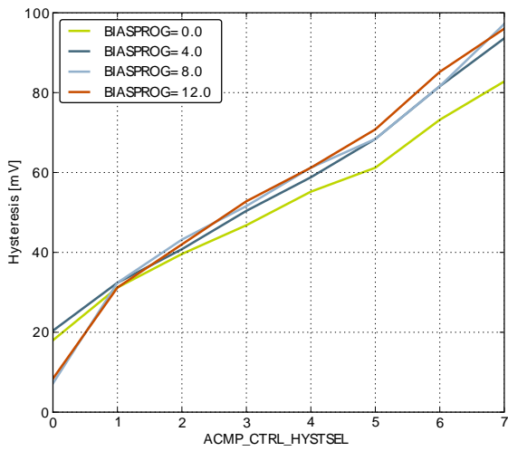
Hysteresis
