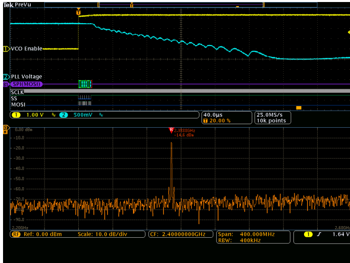
Figure 3 - Spectrum Time is moved another 160 \mu s to the right. At this point the spectrum shows that the PLL has actually overshot the correct frequency and gone all the way down to 2.3888 GHz.
