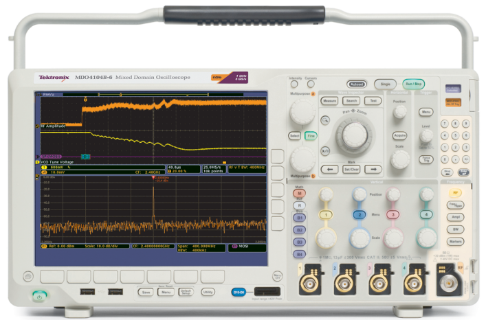
The MDO4000B Series is designed to make your work easier. The large, high-resolution display shows intricate signal details. Dedicated front-panel controls simplify operation. Two USB host ports on the front panel allow you to easily transfer screen shots, instrument settings, and waveform data to a USB mass storage device.
