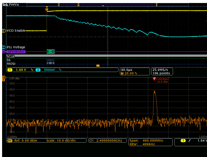
Figure 2 - Spectrum Time is moved about 90 \mu s to the right. At this point, the spectrum shows that the PLL is in the process of tuning to the correct frequency (2.400 GHz). It has made it down to 2.4924 GHz.
