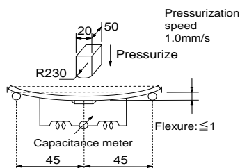
Fig.2 (in mm)
