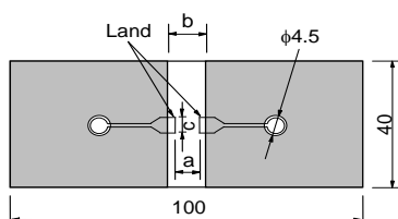
Fig.1 (in mm)
