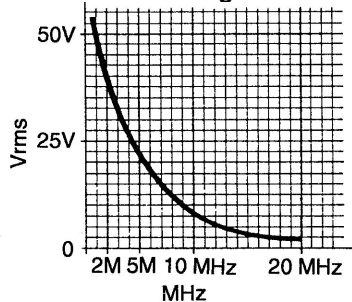
Figure 2. Maximum Signal RF Limits ( V_{\text{rms}} ) at Probe Tip
