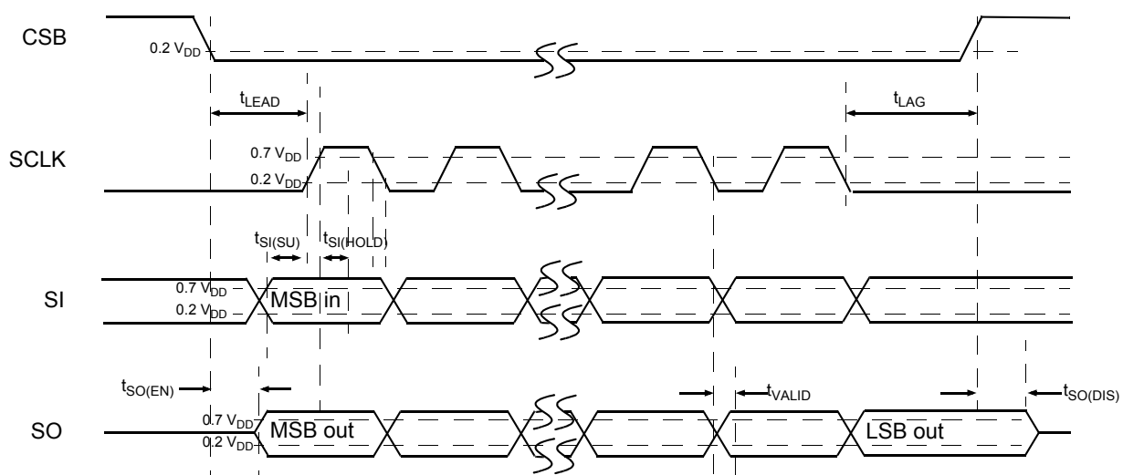
Figure 4. Timing Diagram
