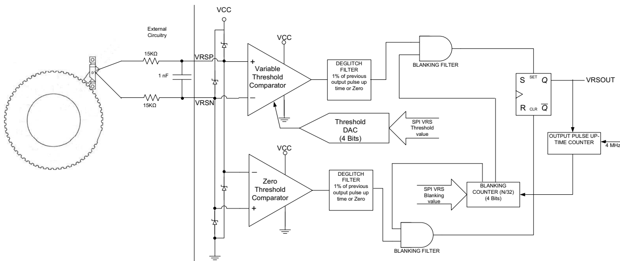
Figure 8. VRS Schematic
