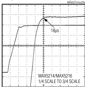
SETTLING TO \pm 0.5 LSB 14 BIT ( V_{DD} = V_{REF} = 5\text{V} , C_L = 100\text{pF} )
