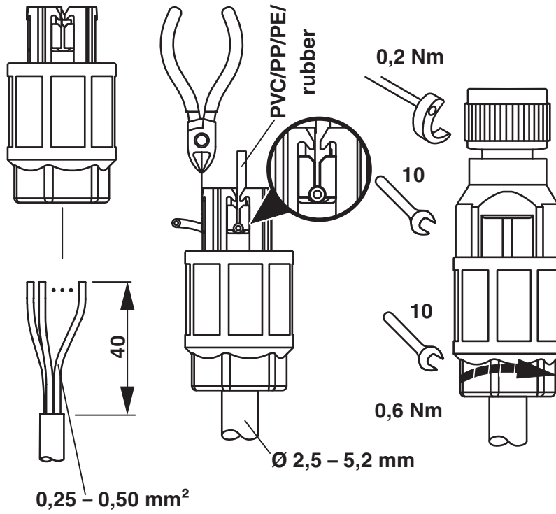
Functional drawing
