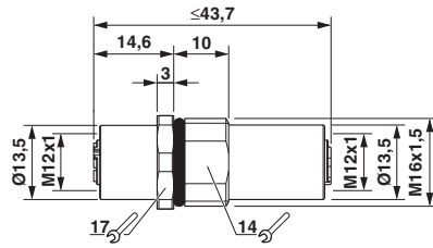
Dimensional drawing
