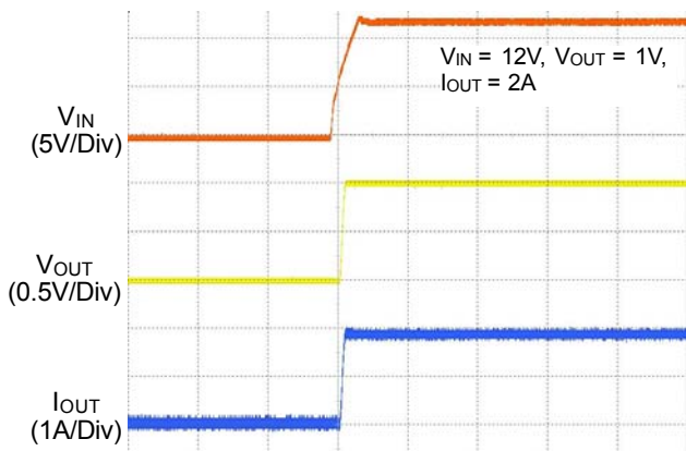
Time (10ms/Div)
