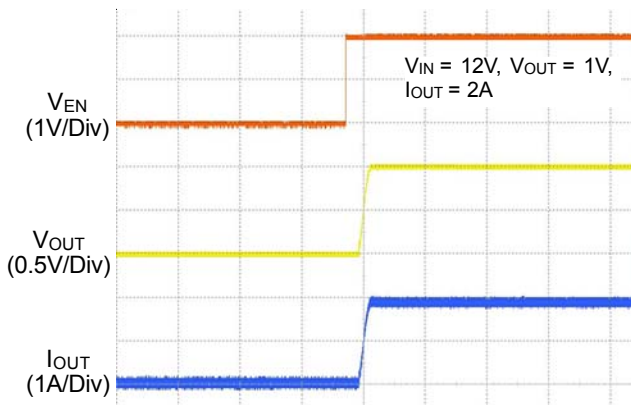
Time (4ms/Div)
