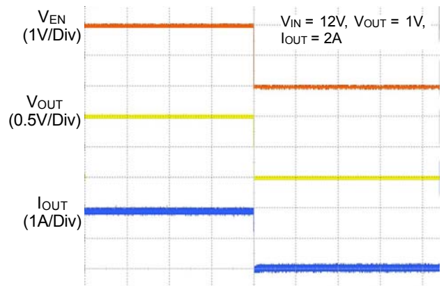
Time (4ms/Div)
