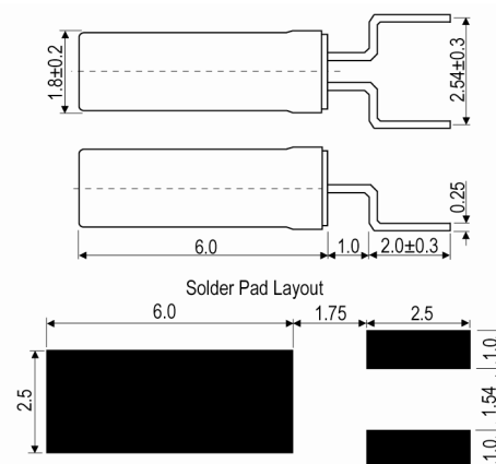
Outline (mm)
