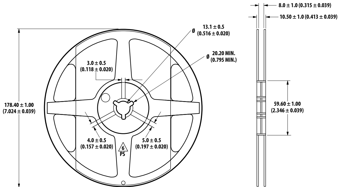
Figure 15. Reel dimensions
