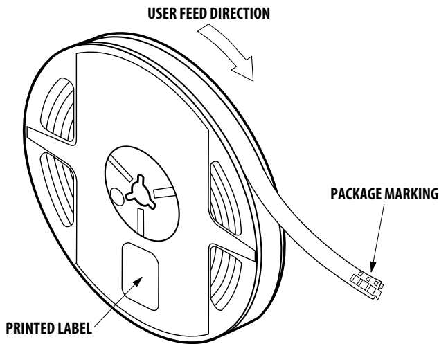
Figure 14. Reeling orientation
