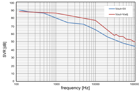
Figure 26: SVR versus frequency
