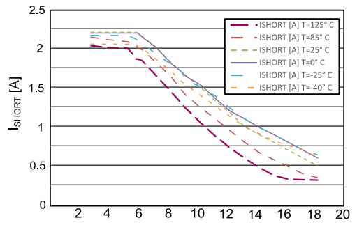
Figure 25: Short-circuit current vs dropout voltage ( V_{OUT} = V_{ADJ} )
