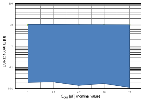
Figure 30: Stability plan ( V_{OUT} = 5\text{ V} )
