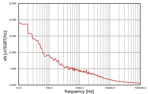
Figure 27: Output noise spectral density ( V_O = V_{ADJ} )
