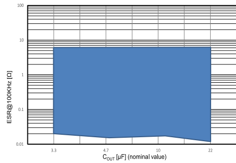
Figure 31: Stability plan ( V_{OUT} = V_{ADJ} )
