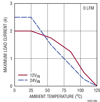
Derating, I-Grade, V_{OUT} = -12\text{V} , BIAS Open, DC2416A Demo Board
