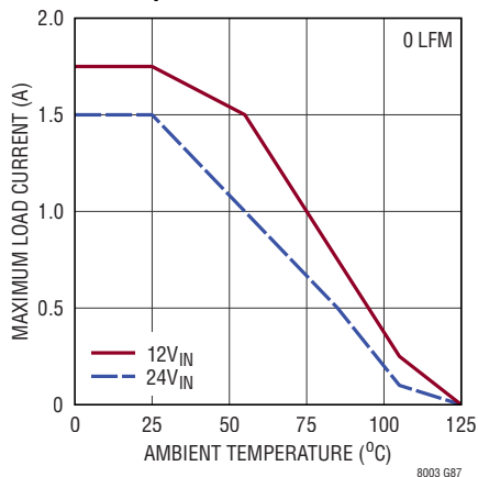
Derating, I-Grade, V_{OUT} = -15\text{V} , BIAS Open, DC2416A Demo Board
