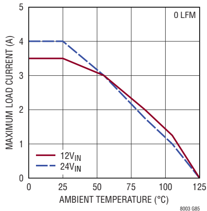
Derating, I-Grade, V_{OUT} = -8\text{V} , BIAS Open, DC2416A Demo Board
