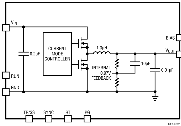
LTM8003-3.3 Block Diagram
