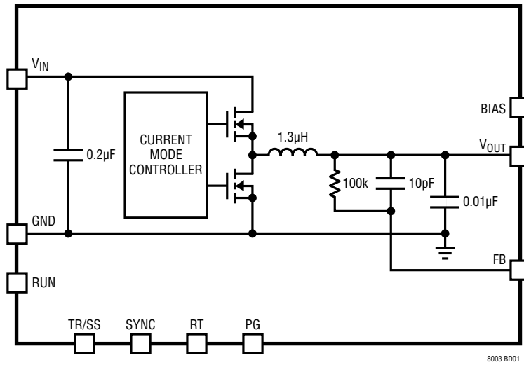
LTM8003 Block Diagram
